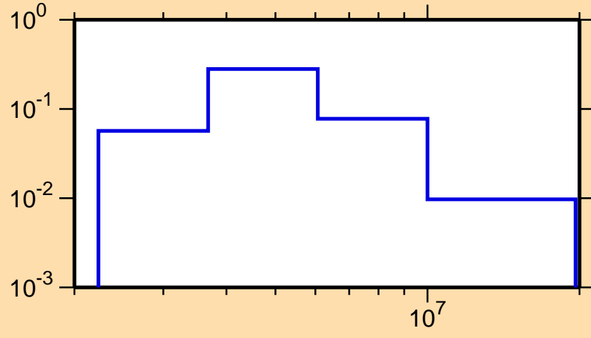
\sigma vs. E for ^{240}\text{Cm}(n,n\text{cont.})
