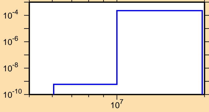
\sigma vs. E for ^{240}\text{Cm}(n,d)
