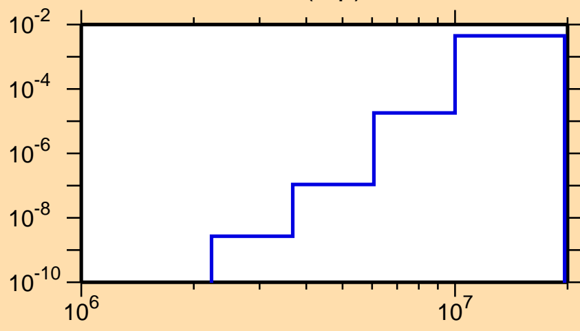
\sigma vs. E for ^{240}\text{Cm}(n,p)
