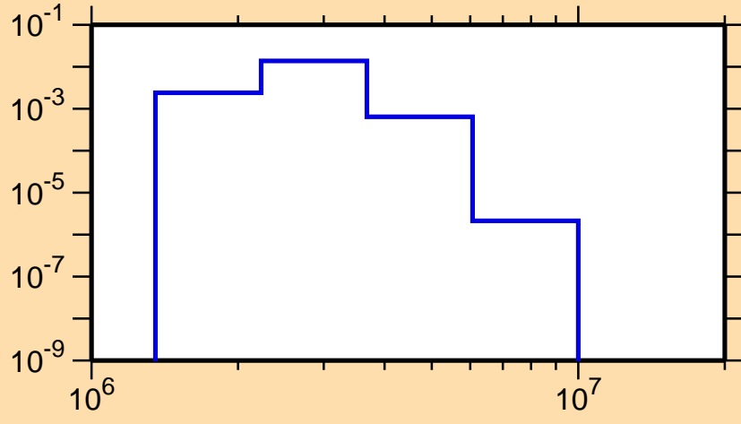
\sigma vs. E for ^{240}\text{Cm}(n,n_2)
