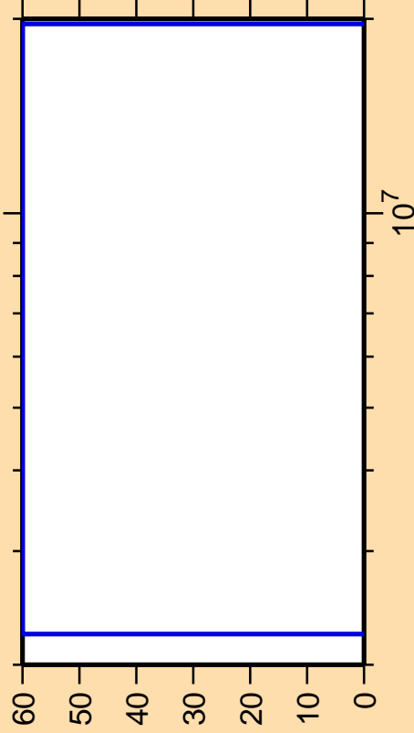
\Delta\sigma/\sigma vs. E for ^{240}\text{Cm}(n,n_{\text{cont}})
