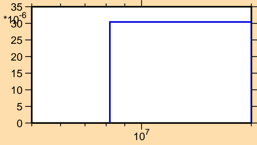
\sigma vs. E for ^{240}\text{Cm}(n,t)
