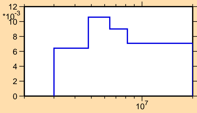
\sigma vs. E for ^{240}\text{Cm}(n,n_3)
