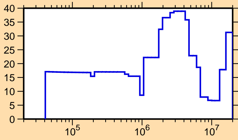
\Delta\sigma/\sigma vs. E for ^{242}\text{Cm}(n,\text{tot.})
