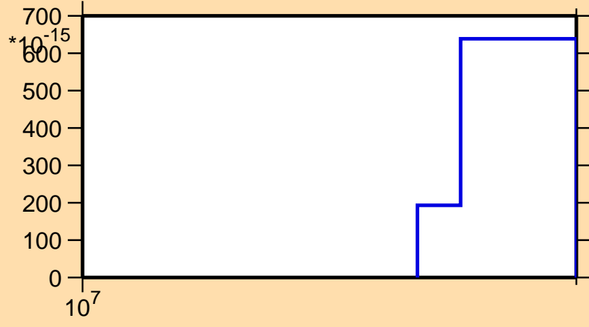
\sigma vs. E for ^{242}\text{Cm}(n,p\alpha)
