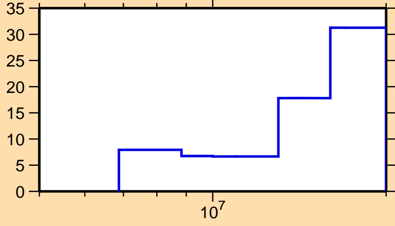
\Delta\sigma/\sigma vs. E for ^{242}\text{Cm}(n,\text{tot.})
