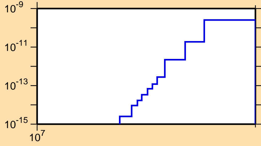
\sigma vs. E for ^{242}\text{Cm}(n,\text{He3})
