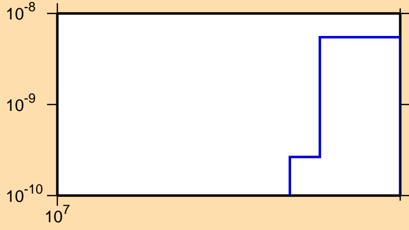
\sigma vs. E for ^{242}\text{Cm}(n,3n\alpha)
