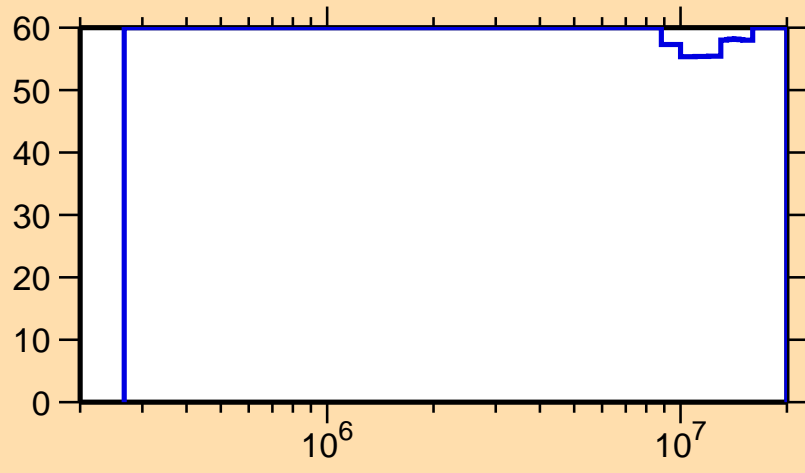
\Delta\sigma/\sigma vs. E for ^{242}\text{Cm}(n,n\text{cont.})
