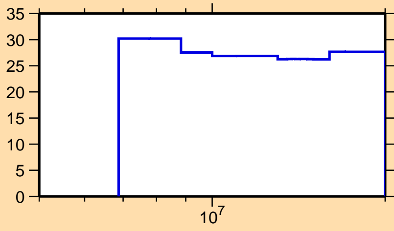
\Delta\sigma/\sigma vs. E for ^{242}\text{Cm}(n,\text{nonel.})
