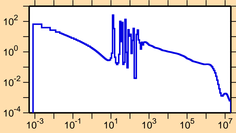
\sigma vs. E for ^{242}\text{Cm}(n,\gamma)
