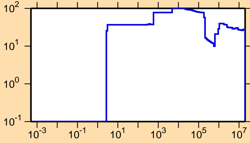
\Delta\sigma/\sigma vs. E for ^{242}\text{Cm}(n,\text{nonel.})
