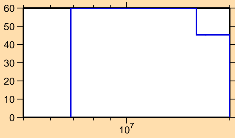
\Delta\sigma/\sigma vs. E for ^{242}\text{Cm}(n,2n)
