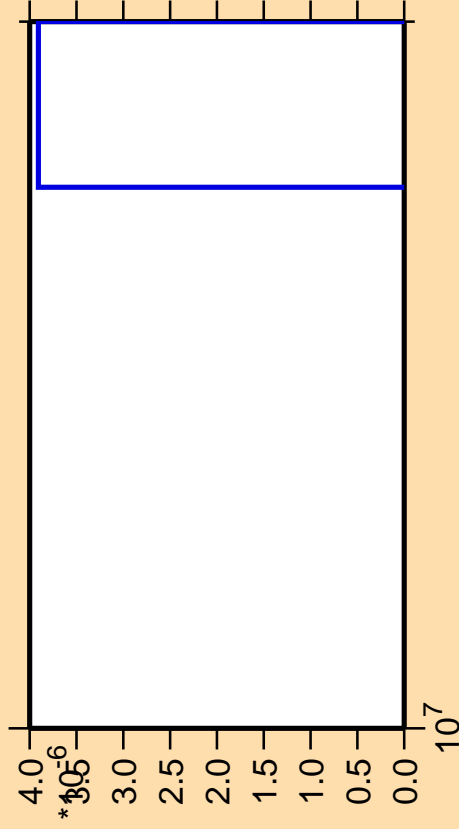
\Delta\sigma/\sigma vs. E for ^{242}\text{Cm} (mt 42)
