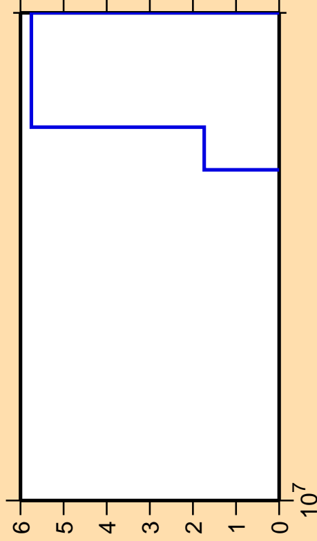
\Delta\sigma/\sigma vs. E for ^{242}\text{Cm}(n,p\alpha)
