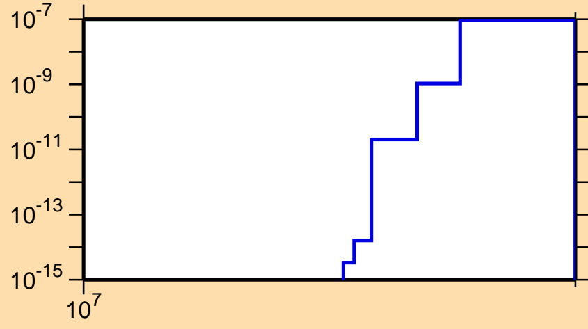
\sigma vs. E for ^{242}\text{Cm}(n,2np)
