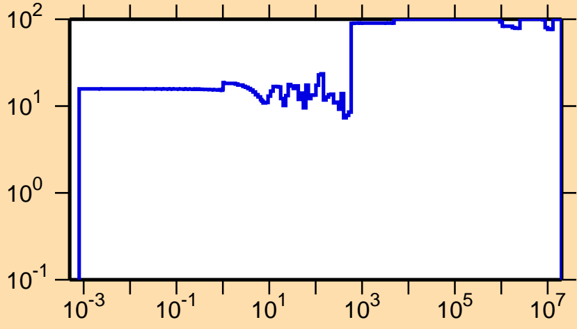
\Delta\sigma/\sigma vs. E for ^{242}\text{Cm}(n,\gamma)
