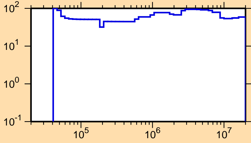
\Delta\sigma/\sigma vs. E for ^{242}\text{Cm}(n,\text{inel.})
