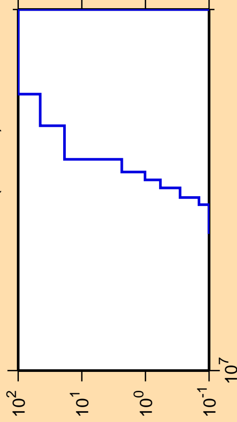
\Delta\sigma/\sigma vs. E for ^{242}\text{Cm}(n,\text{He3})
