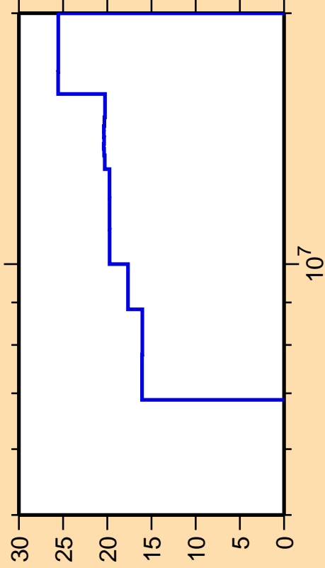
\Delta\sigma/\sigma vs. E for ^{242}\text{Cm}(n,f)
