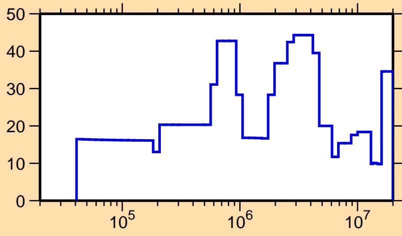
\Delta\sigma/\sigma vs. E for ^{242}\text{Cm}(n,\text{el.})
