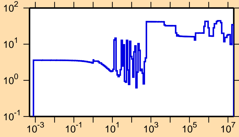
\Delta\sigma/\sigma vs. E for ^{242}\text{Cm}(n,el.)
