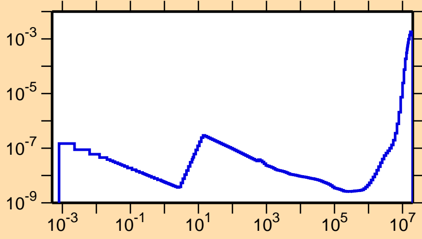
\sigma vs. E for ^{242}\text{Cm}(n,\alpha)
