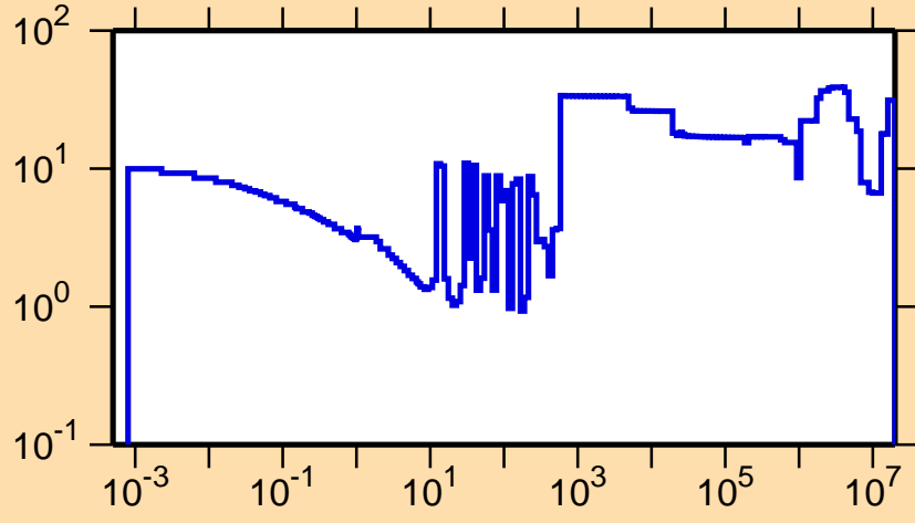
\Delta\sigma/\sigma vs. E for ^{242}\text{Cm}(n,tot.)
