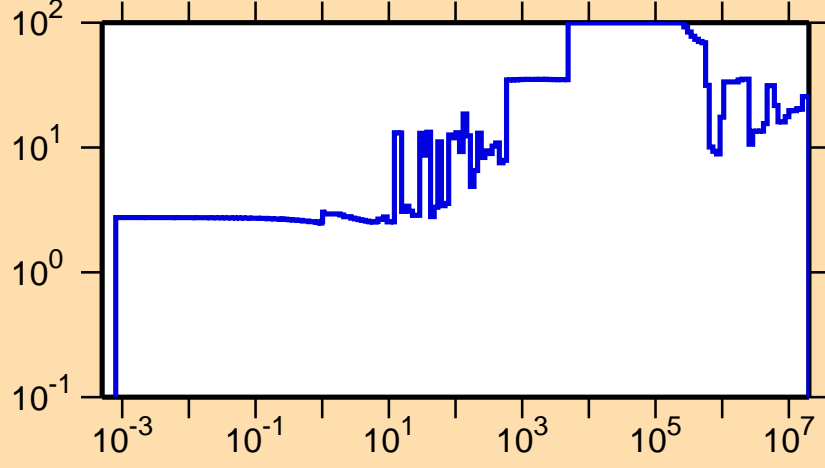
\Delta\sigma/\sigma vs. E for ^{242}\text{Cm}(n,f)
