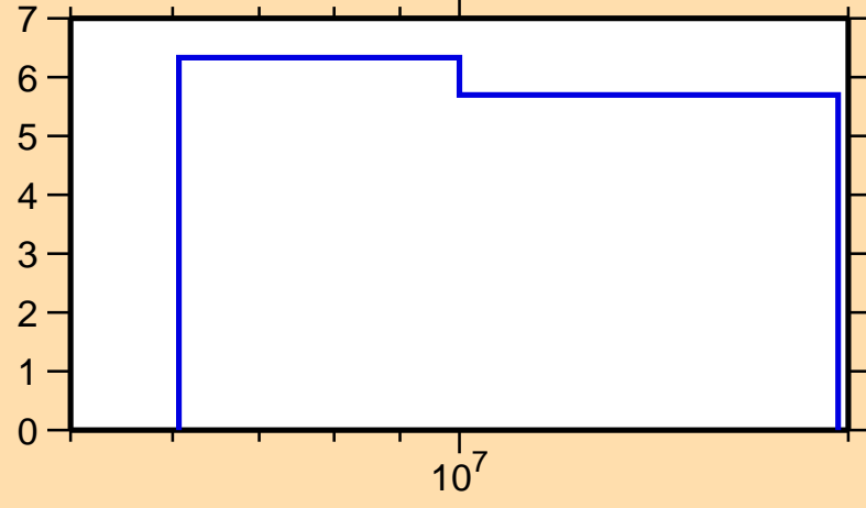
\Delta\sigma/\sigma vs. E for ^{242}\text{Cm}(n,\text{el.})
