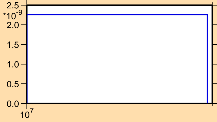
\sigma vs. E for ^{242}\text{Cm}(n,nd)
