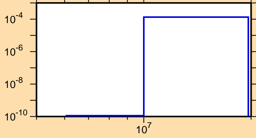
\sigma vs. E for ^{242}\text{Cm}(n,d)
