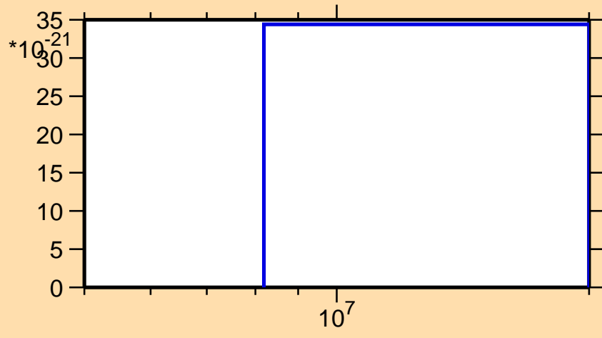
\sigma vs. E for ^{242}\text{Cm} (mt 42)
