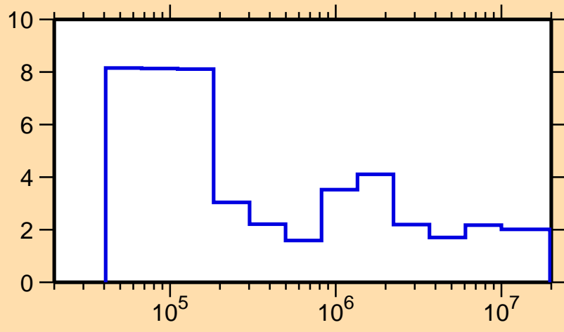
\Delta\sigma/\sigma vs. E for ^{243}\text{Cm}(n,\text{nonel.})
