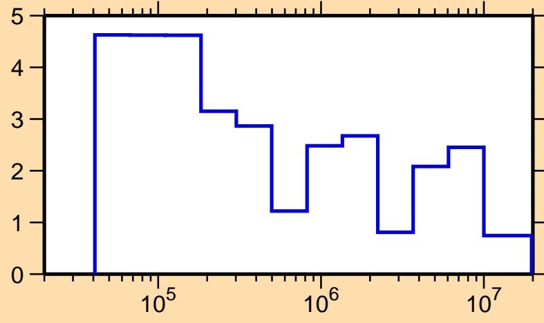
\Delta\sigma/\sigma vs. E for ^{243}\text{Cm}(n,\text{el.})
