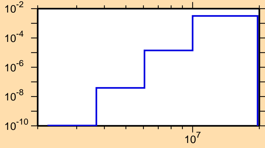
\sigma vs. E for ^{243}\text{Cm}(n,p)
