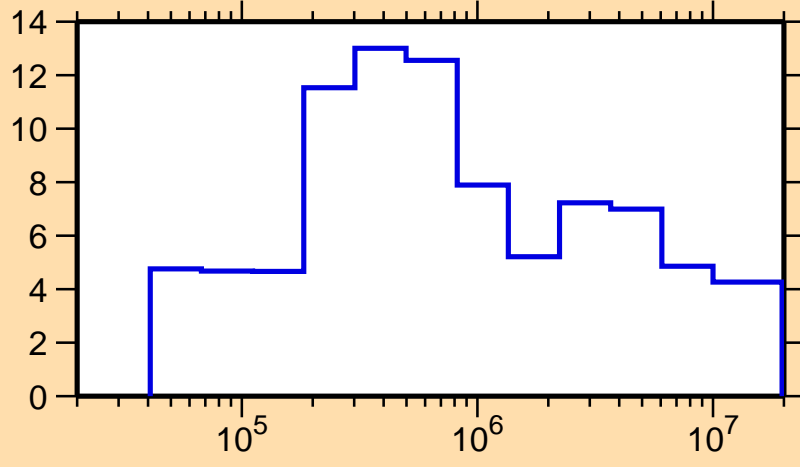
\Delta\sigma/\sigma vs. E for ^{243}\text{Cm}(n,n_1)
