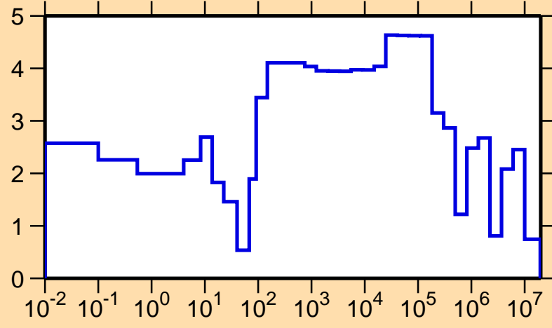
\Delta\sigma/\sigma vs. E for ^{243}\text{Cm}(n,el.)
