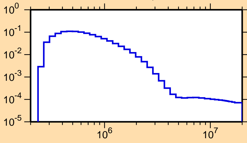
\sigma vs. E for ^{245}\text{Cm}(n,n_4)
