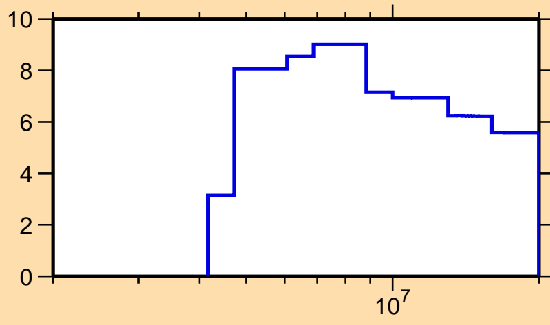
\Delta\sigma/\sigma vs. E for ^{245}\text{Cm}(n,p)
