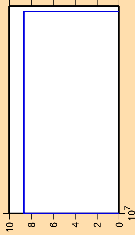
\Delta\sigma/\sigma vs. E for ^{245}\text{Cm}(n,nd)
