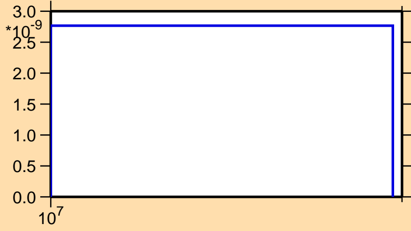
\sigma vs. E for ^{245}\text{Cm}(n,2np)
