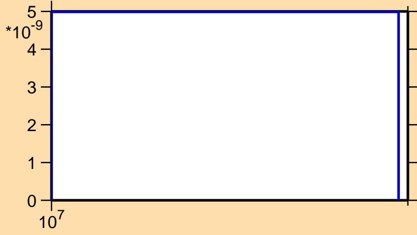
\sigma vs. E for ^{245}\text{Cm}(n,nt)
