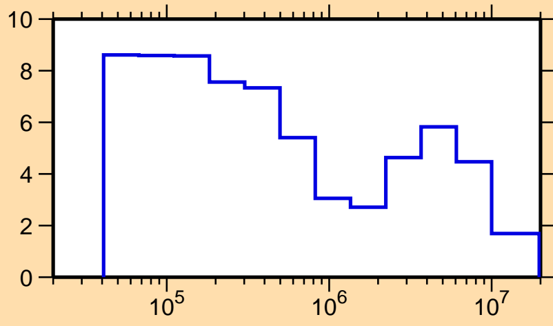
\Delta\sigma/\sigma vs. E for ^{245}\text{Cm}(n,f)
