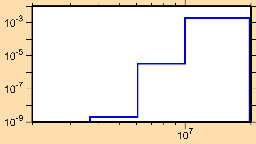
\sigma vs. E for ^{245}\text{Cm}(n,p)
