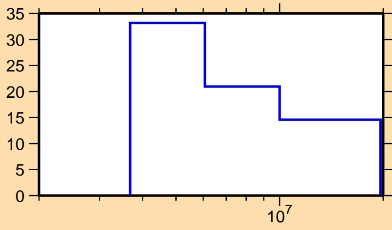
\Delta\sigma/\sigma vs. E for ^{245}\text{Cm}(n,2n)
