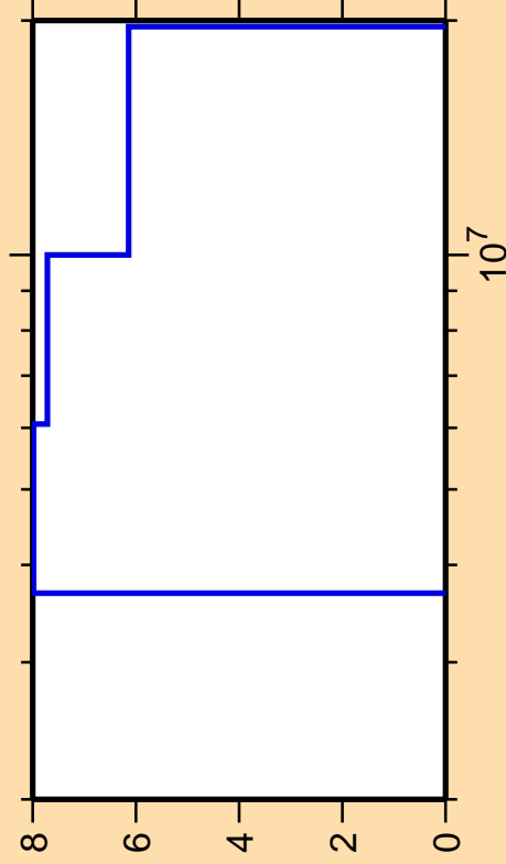
\Delta\sigma/\sigma vs. E for ^{245}\text{Cm}(n,p)
