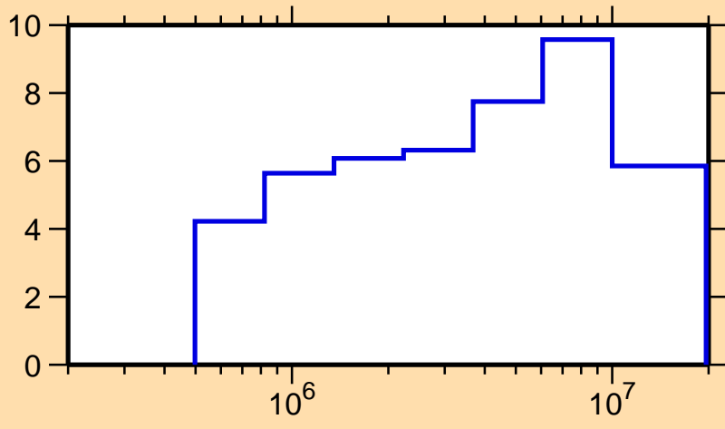
\Delta\sigma/\sigma vs. E for ^{245}\text{Cm}(n,n\text{cont.})
