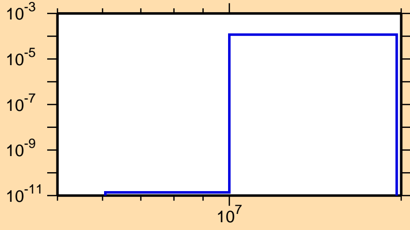
\sigma vs. E for ^{245}\text{Cm}(n,d)
