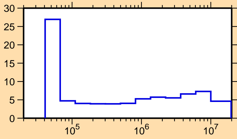
\Delta\sigma/\sigma vs. E for ^{245}\text{Cm}(n,\text{inel.})
