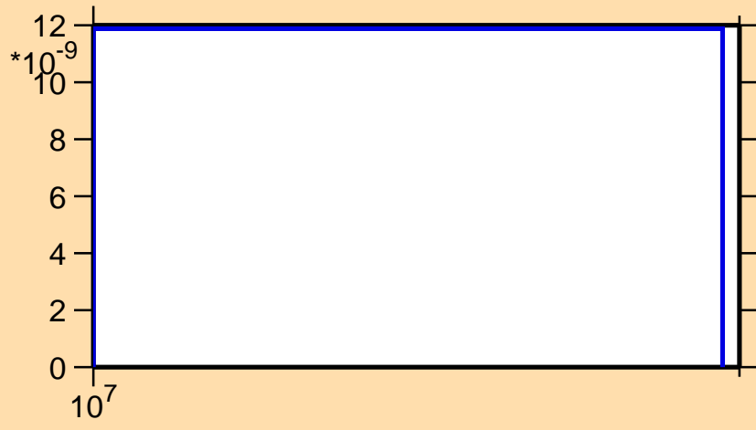
\sigma vs. E for ^{245}\text{Cm}(n,nd)
