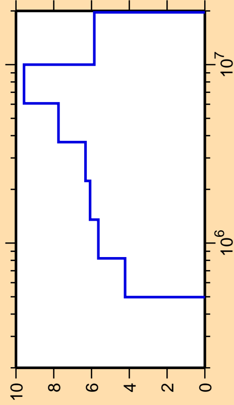
\Delta\sigma/\sigma vs. E for ^{245}\text{Cm}(n,\text{ncont.})
