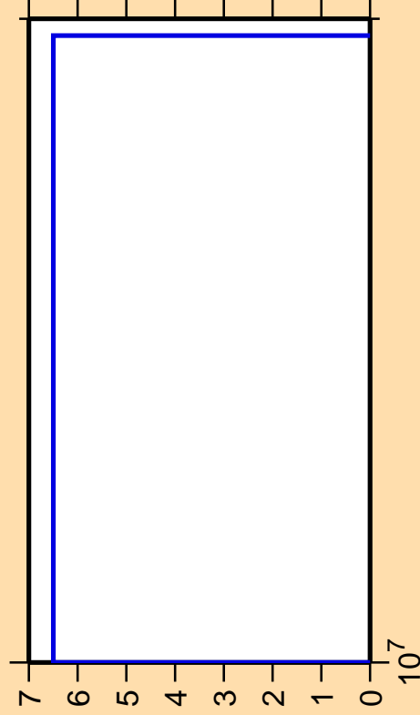
\Delta\sigma/\sigma vs. E for ^{245}\text{Cm}(n,nt)
