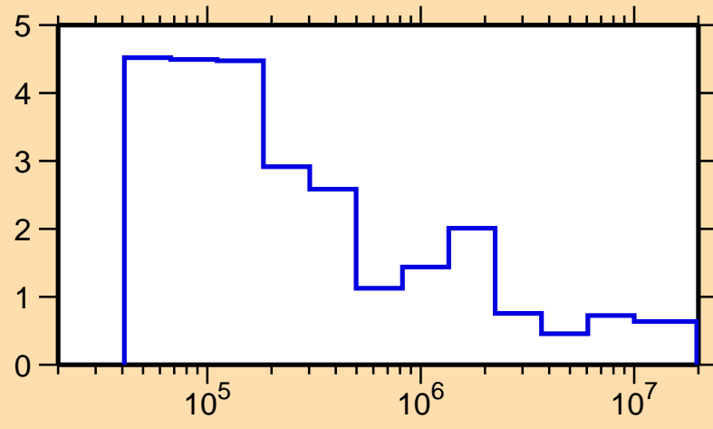
\Delta\sigma/\sigma vs. E for ^{245}\text{Cm}(n,\text{nonel.})
