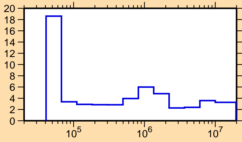
\Delta\sigma/\sigma vs. E for ^{245}\text{Cm}(n,n_1)
