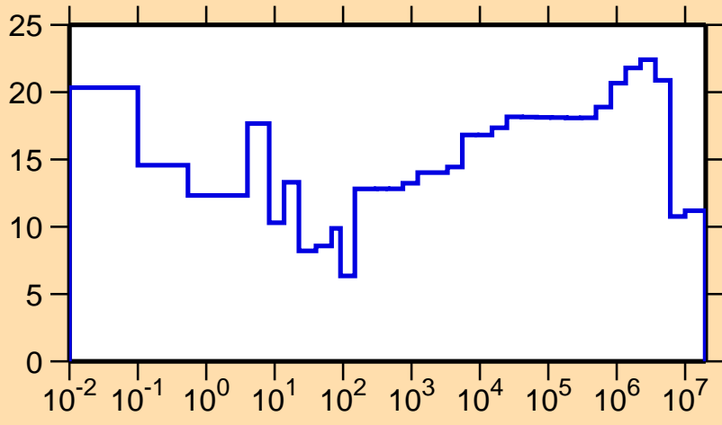
\Delta\sigma/\sigma vs. E for ^{245}\text{Cm}(n,\gamma)
