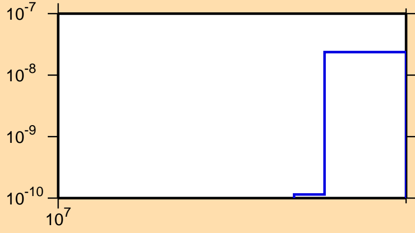
\sigma vs. E for ^{246}\text{Cm}(n,2np)
