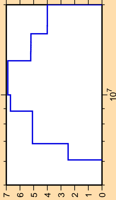
\Delta\sigma/\sigma vs. E for ^{246}\text{Cm}(n,p)
