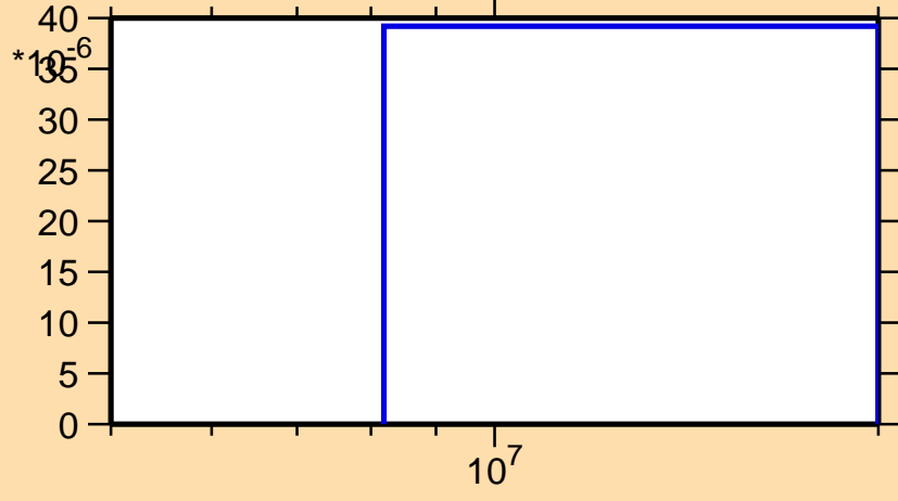
\sigma vs. E for ^{247}\text{Cm}(n,d)
