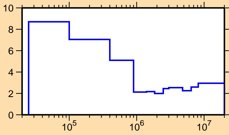
\Delta\sigma/\sigma vs. E for ^{247}\text{Cm}(n,n_1)
