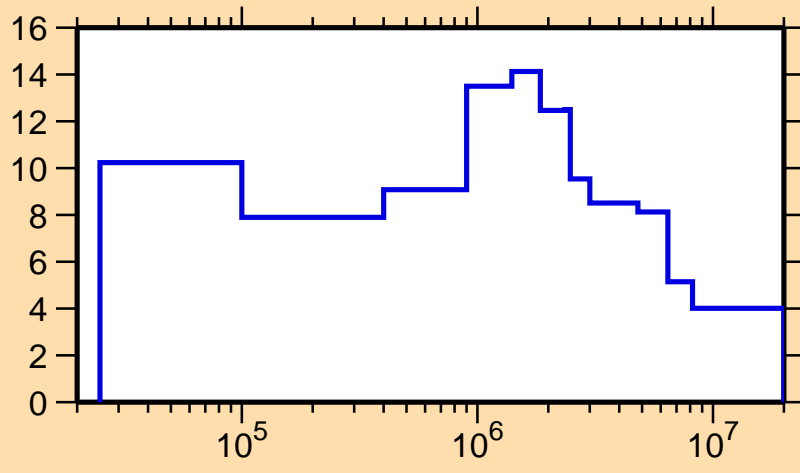
\Delta\sigma/\sigma vs. E for ^{247}\text{Cm}(n,inel.)
