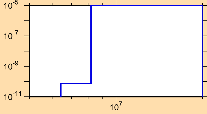
\sigma vs. E for ^{247}\text{Cm}(n,n\alpha)
