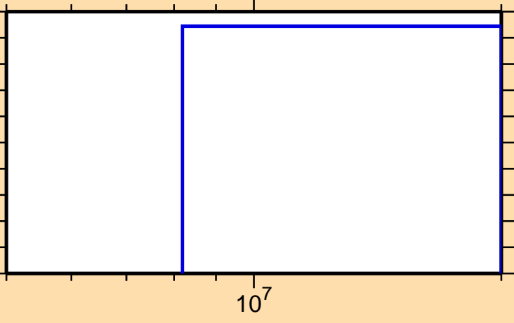
\sigma vs. E for ^{247}\text{Cm}(n,t)
