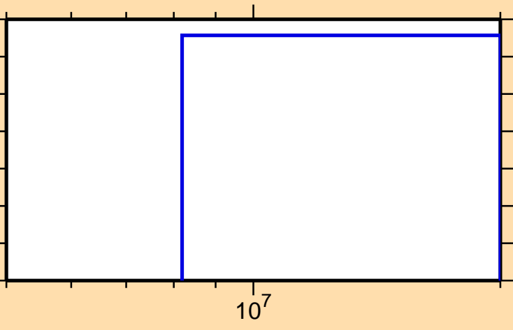
\sigma vs. E for ^{247}\text{Cm}(n,nt)
