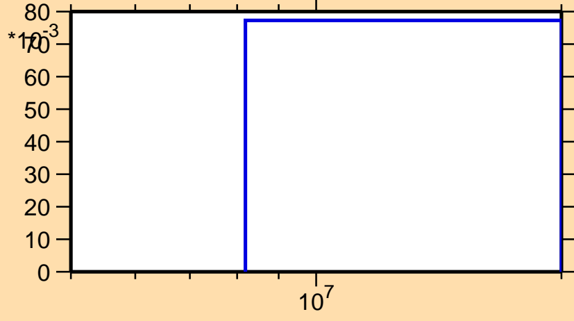
\sigma vs. E for ^{247}\text{Cm}(n,3n)
