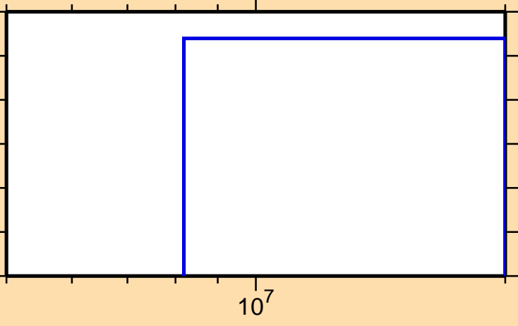
\sigma vs. E for ^{247}\text{Cm}(n,2np)
