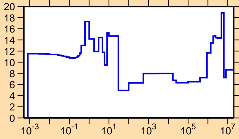
\Delta\sigma/\sigma vs. E for ^{247}\text{Cm}(n,\gamma)
