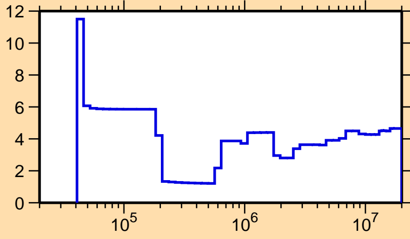
\Delta\sigma/\sigma vs. E for ^{248}\text{Cm}(n,n_1)
