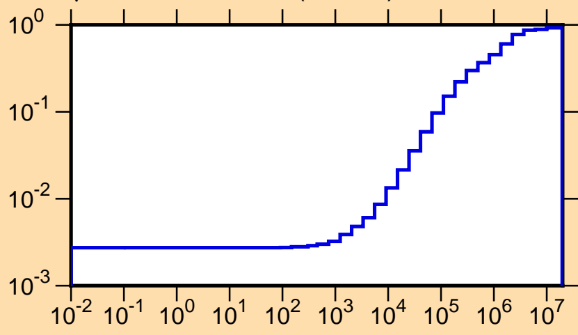
\mu vs. E for ^{248}\text{Cm}(\text{mt251})
