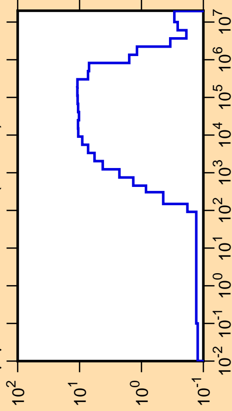
\Delta\mu/\mu vs. E for ^{248}\text{Cm}(\text{mt251})
