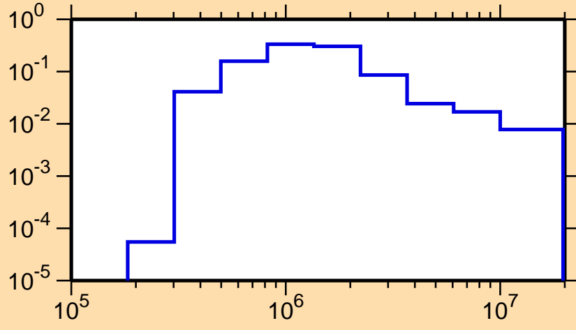
\sigma vs. E for ^{250}\text{Cm}(n,n_2)
