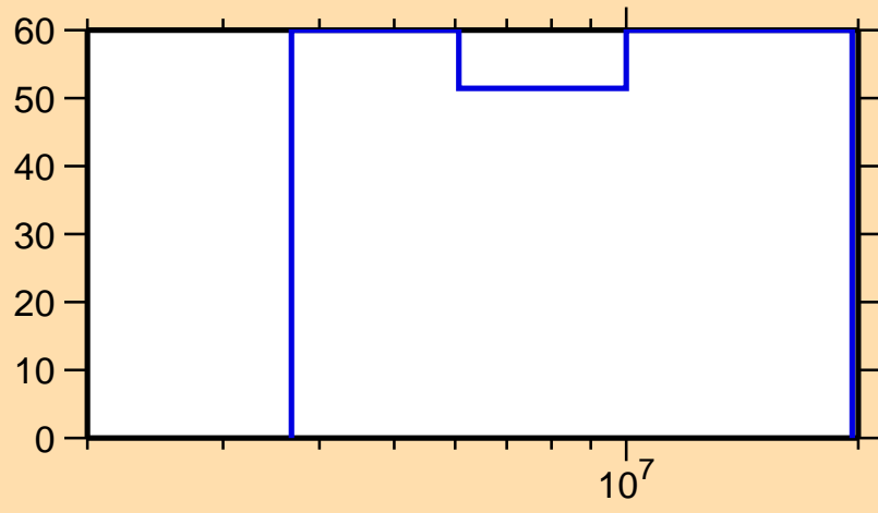
\Delta\sigma/\sigma vs. E for ^{250}\text{Cm}(n,2n)
