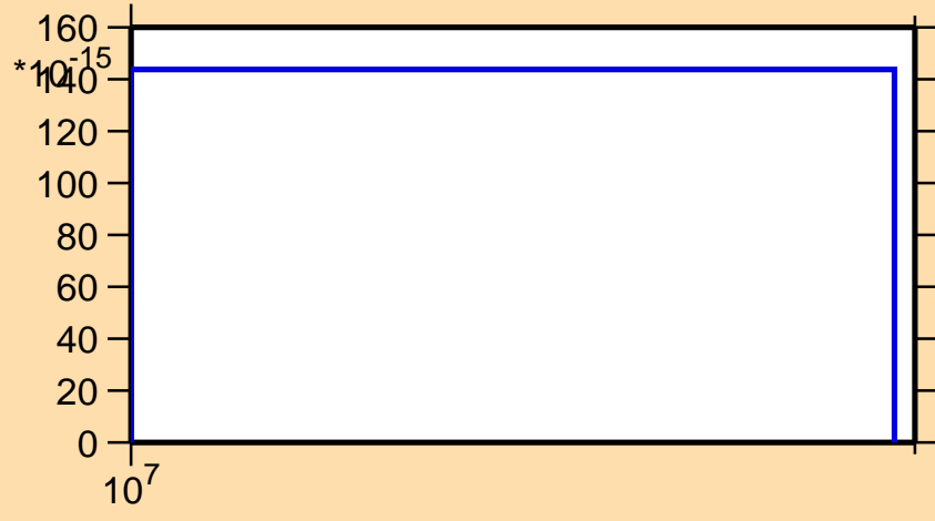
\sigma vs. E for ^{250}\text{Cm}(n,3n\alpha)
