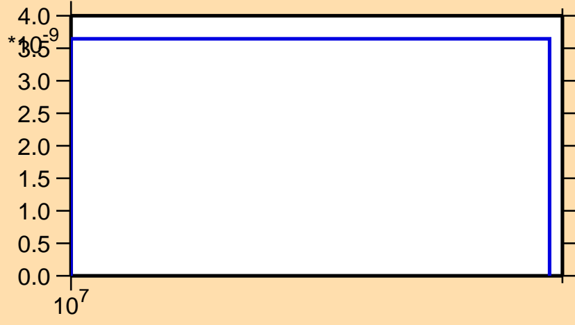
\sigma vs. E for ^{250}\text{Cm}(n,2n\alpha)
