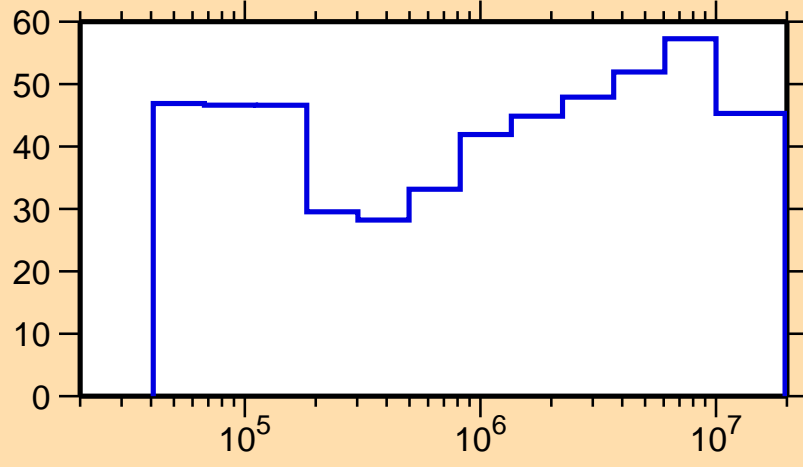
\Delta\sigma/\sigma vs. E for ^{250}\text{Cm}(n,n_1)
