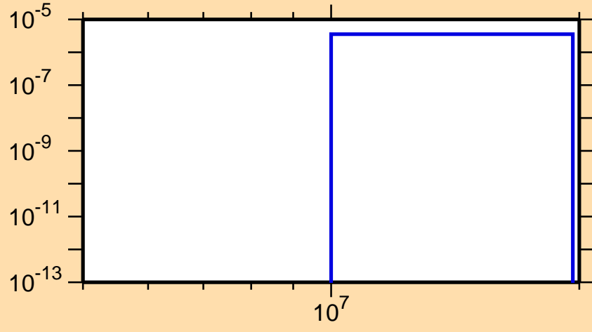
\sigma vs. E for ^{250}\text{Cm}(n,np)
