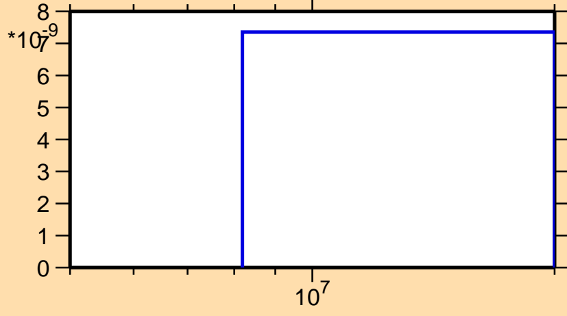
\sigma vs. E for ^{250}\text{Cm}(n,nt)
