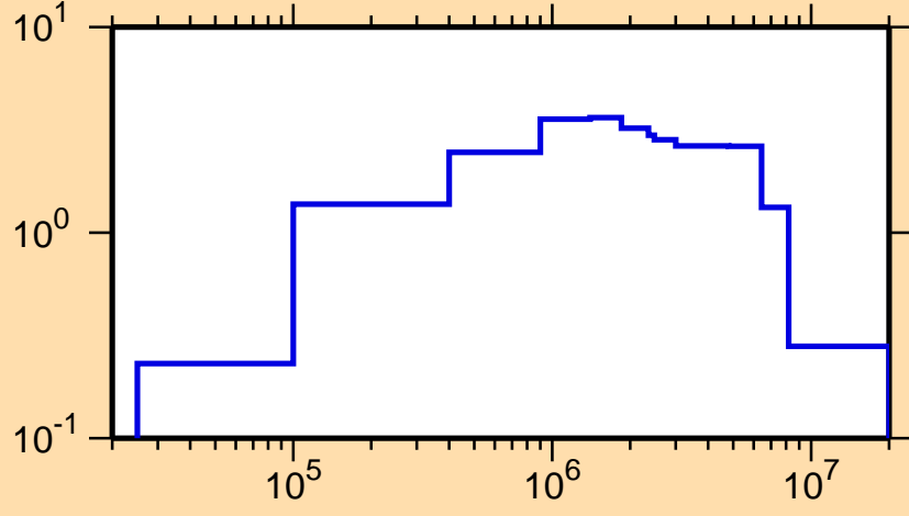
\sigma vs. E for ^{250}\text{Cm}(n,\text{inel.})
