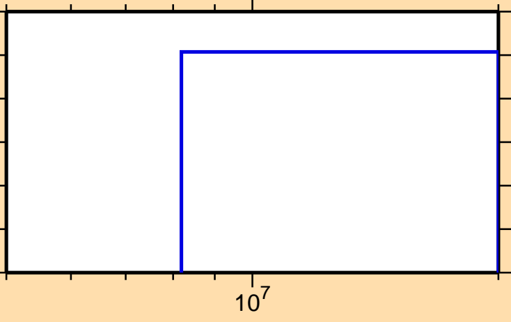
\sigma vs. E for ^{250}\text{Cm}(n,t)
