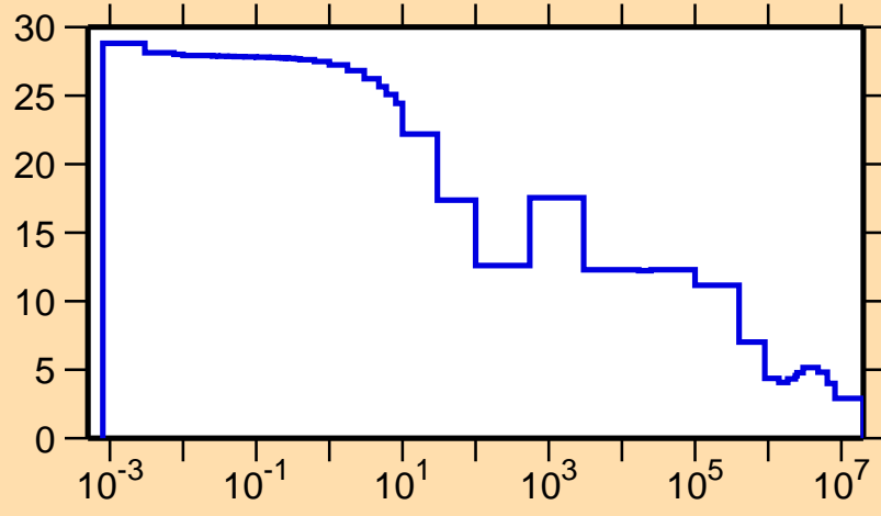
\sigma vs. E for ^{250}\text{Cm}(n,\text{el.})
