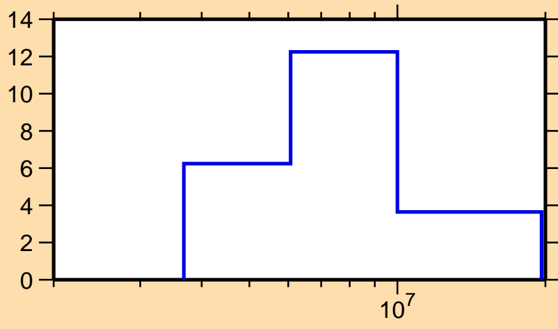
\Delta\sigma/\sigma vs. E for ^{251}\text{Cm}(n,\text{tot.})
