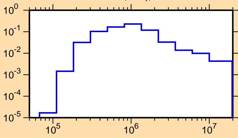
\sigma vs. E for ^{251}\text{Cm}(n,n_1)
