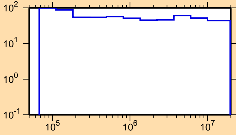
\Delta\sigma/\sigma vs. E for ^{251}\text{Cm}(n,n_1)
