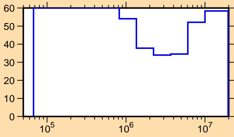
\Delta\sigma/\sigma vs. E for ^{251}\text{Cm}(n,\text{inel.})
