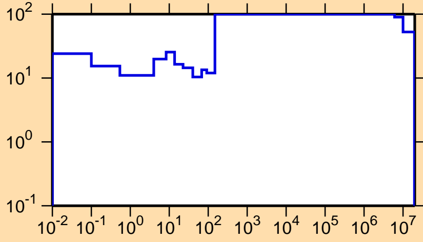
\Delta\sigma/\sigma vs. E for ^{251}\text{Cm}(n, \gamma)
