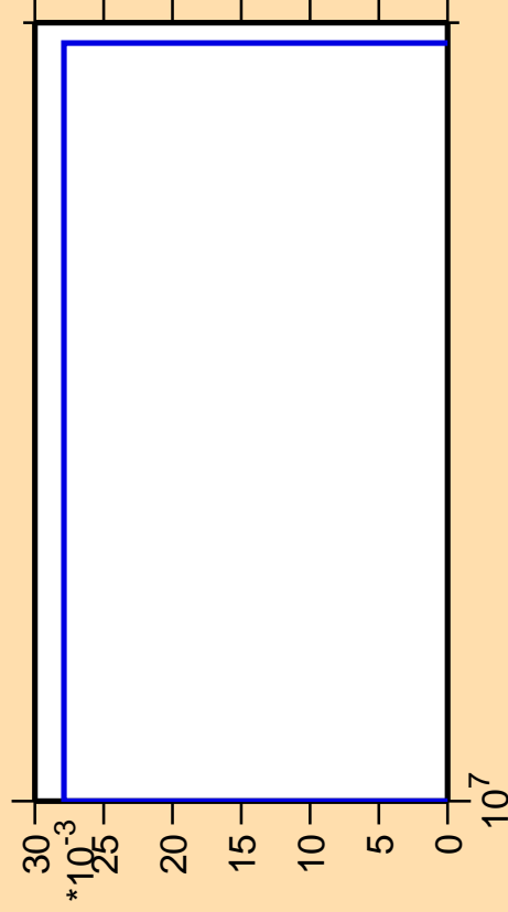
\Delta\sigma/\sigma vs. E for ^{251}\text{Cm}(n,\text{He}3)
