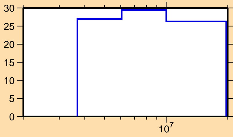
\Delta\sigma/\sigma vs. E for ^{251}\text{Cm}(n,2n)
