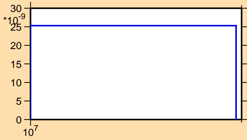
\sigma vs. E for ^{251}\text{Cm}(n,nt)
