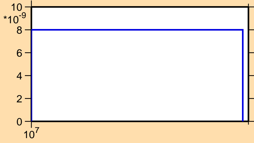
\sigma vs. E for ^{251}\text{Cm}(n,nd)
