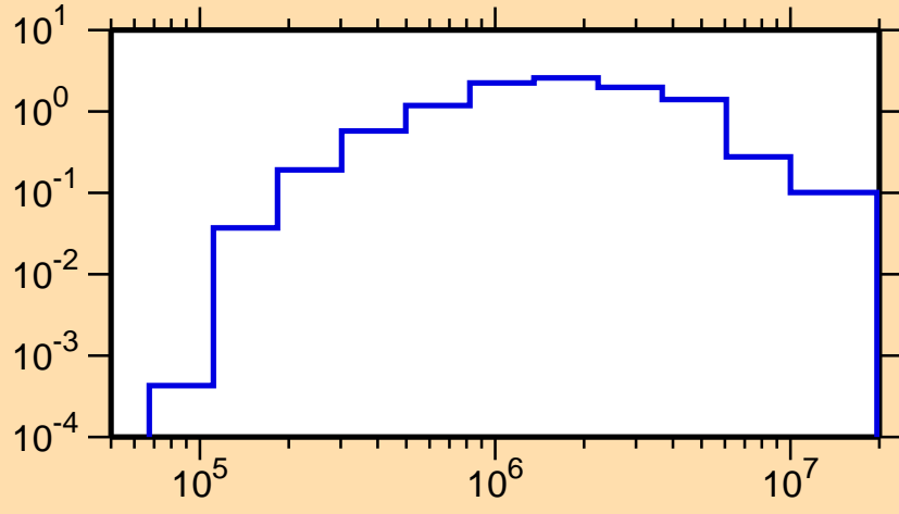
\sigma vs. E for ^{251}\text{Cm}(n,\text{inel.})
