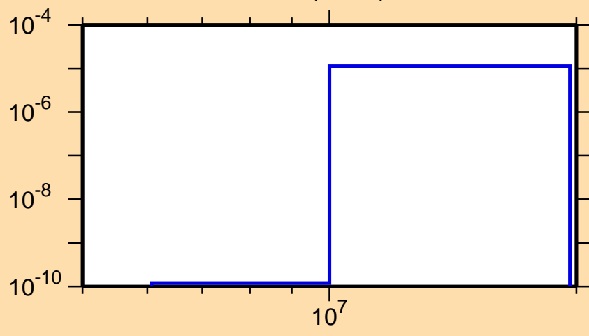
\sigma vs. E for ^{251}\text{Cm}(n,n\alpha)
