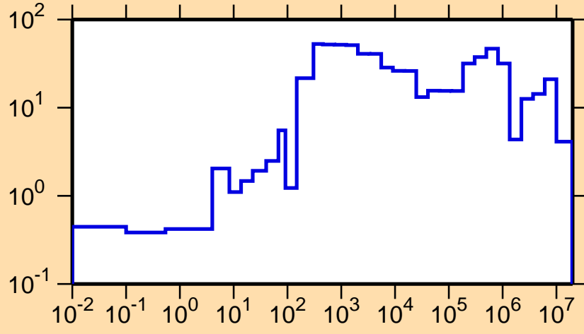
\Delta\sigma/\sigma vs. E for ^{251}\text{Cm}(n,el.)
