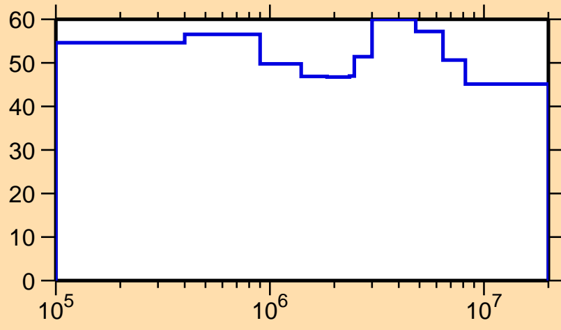
\Delta\sigma/\sigma vs. E for ^{251}\text{Cm}(n,n_1)
