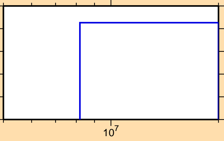
\sigma vs. E for ^{251}\text{Cm}(n,np)
