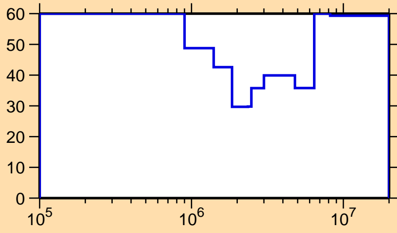
\Delta\sigma/\sigma vs. E for ^{251}\text{Cm}(n,n\text{cont.})
