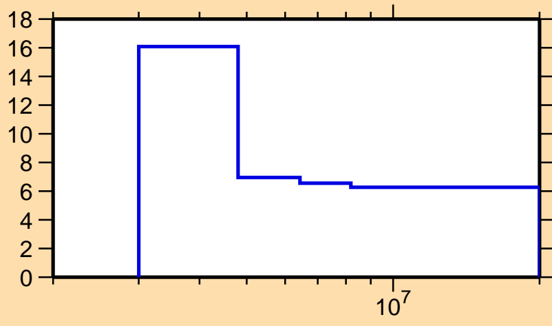
\Delta\sigma/\sigma vs. E for ^{251}\text{Cm}(n,\text{nonel.})
