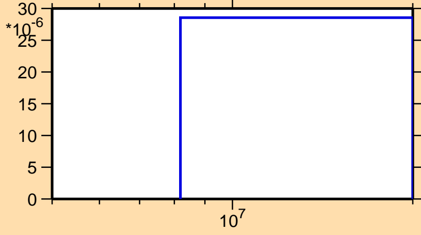
\sigma vs. E for ^{251}\text{Cm}(n,d)
