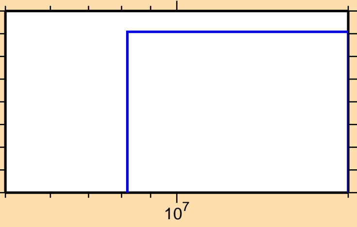
\sigma vs. E for ^{251}\text{Cm}(n,nd)
