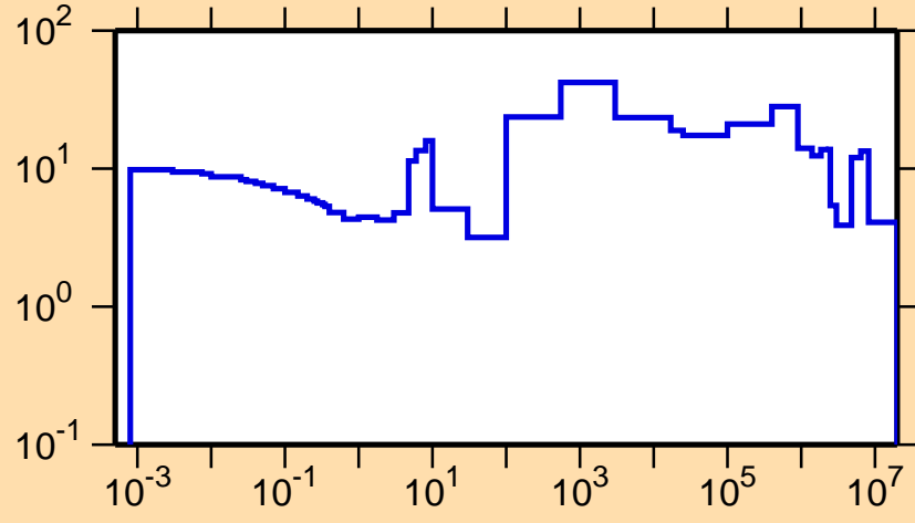
\Delta\sigma/\sigma vs. E for ^{251}\text{Cm}(n,tot.)
