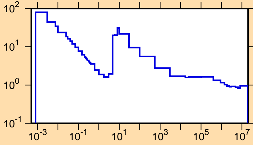
\sigma vs. E for ^{251}\text{Cm}(n,f)
