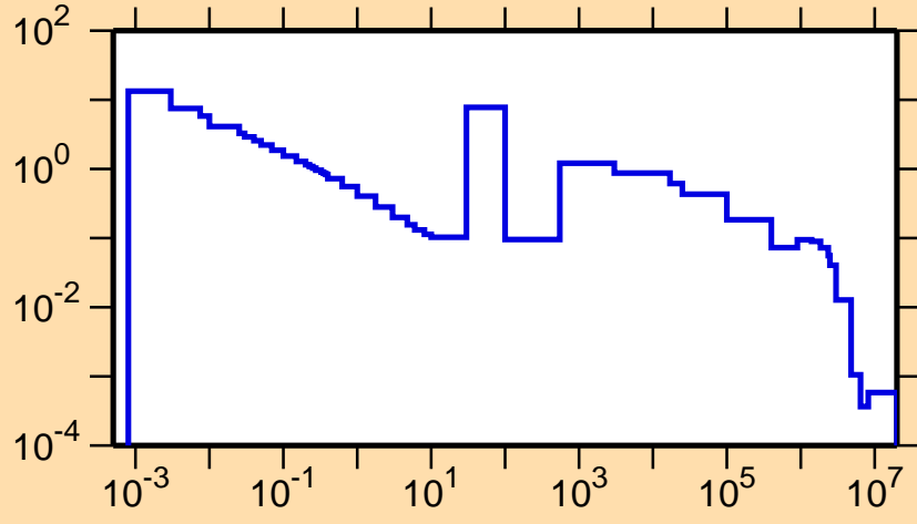
\sigma vs. E for ^{252}\text{Cm}(n,\gamma)
