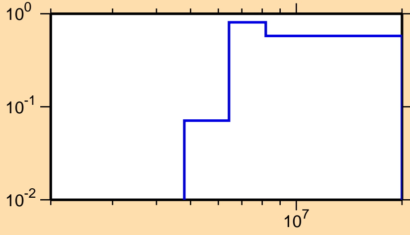
\sigma vs. E for ^{252}\text{Cm}(n,2n)
