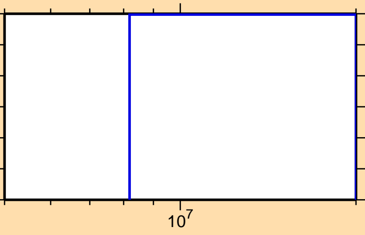
\sigma vs. E for ^{252}\text{Cm}(n,nt)
