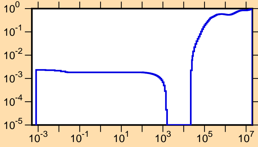
\mu vs. E for ^{285}
