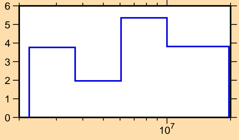
\Delta\sigma/\sigma vs. E for ^{54}\text{Co}(n,\text{tot.})
