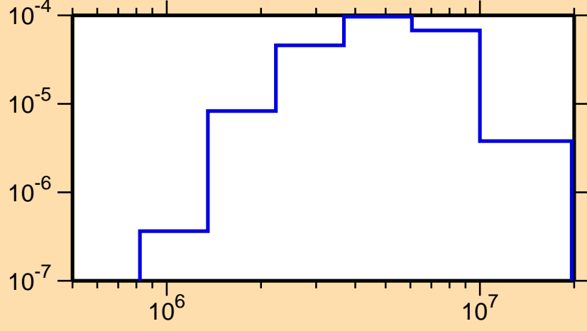
\sigma vs. E for ^{54}\text{Co}(n,n_2)
