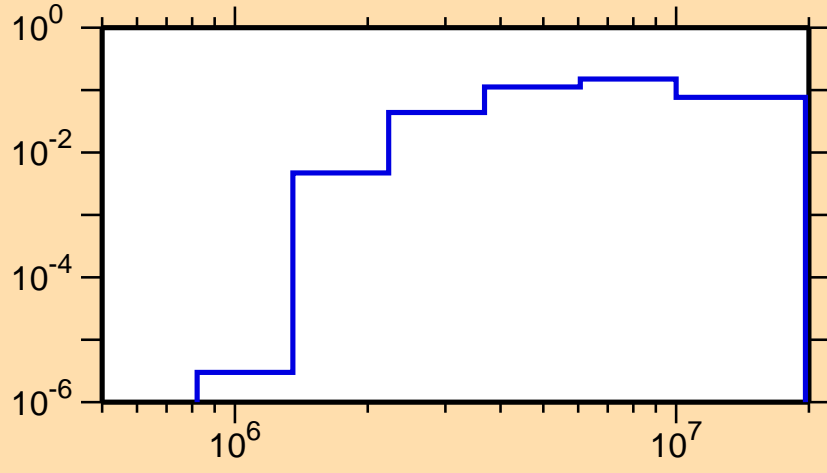
\sigma vs. E for ^{54}\text{Co}(n,\text{inel.})
