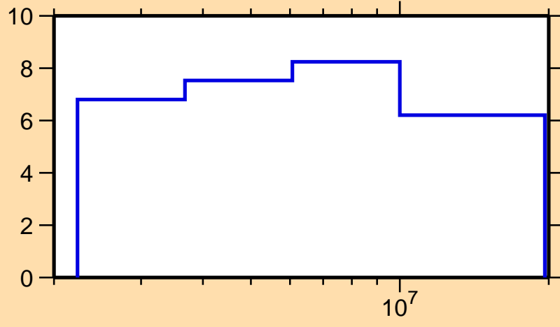
\Delta\sigma/\sigma vs. E for ^{54}\text{Co}(n,n\text{nonel.})
