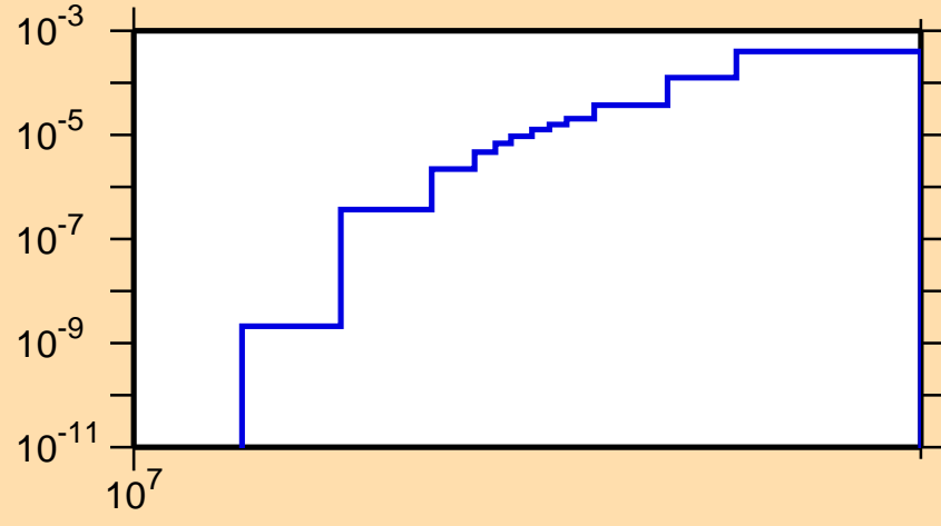
\sigma vs. E for ^{55}\text{Co}(n,t)
