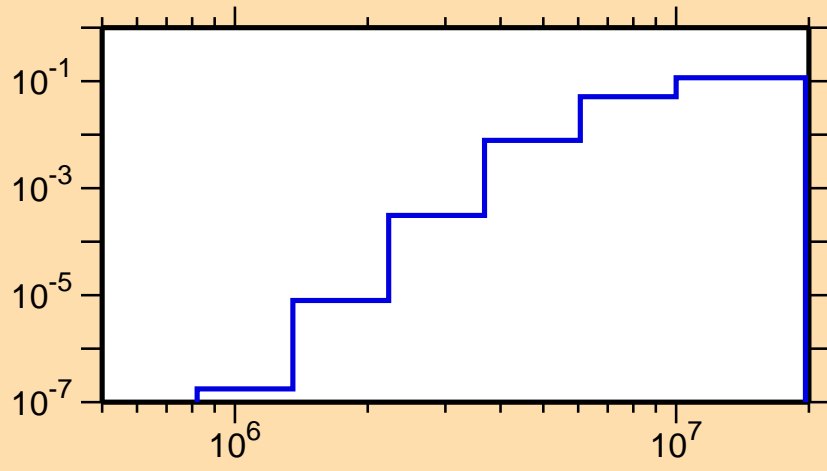
\sigma vs. E for ^{55}\text{Co}(n,\alpha)
