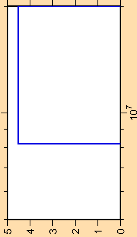
\Delta\sigma/\sigma vs. E for ^{55}\text{Co} (mt 45)
