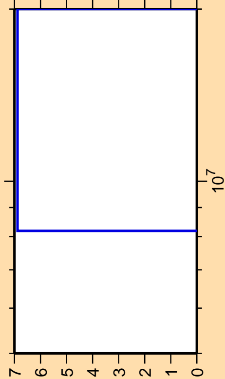
\Delta\sigma/\sigma vs. E for ^{55}\text{Co}(\text{mt117})
