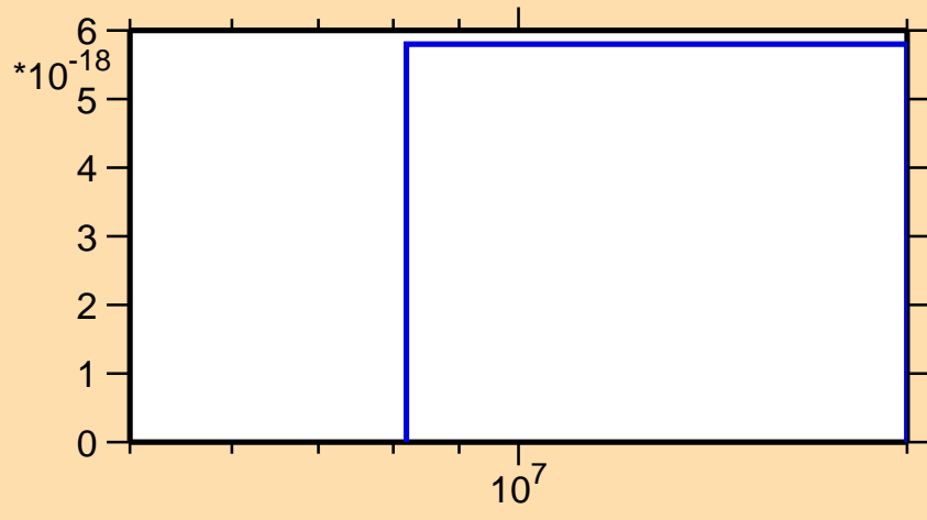
\sigma vs. E for ^{55}\text{Co} (mt 34)
