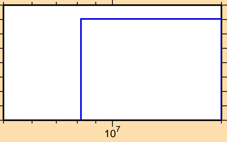
\sigma vs. E for ^{55}\text{Co}(n,n\alpha)
