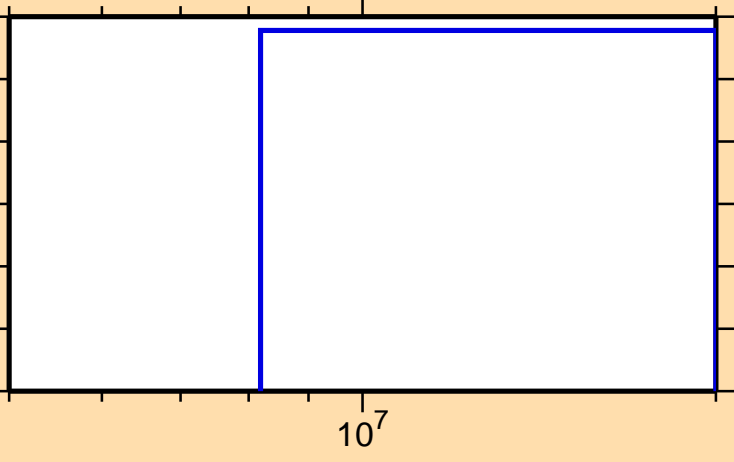
\sigma vs. E for ^{55}\text{Co}(n,\text{pd})
