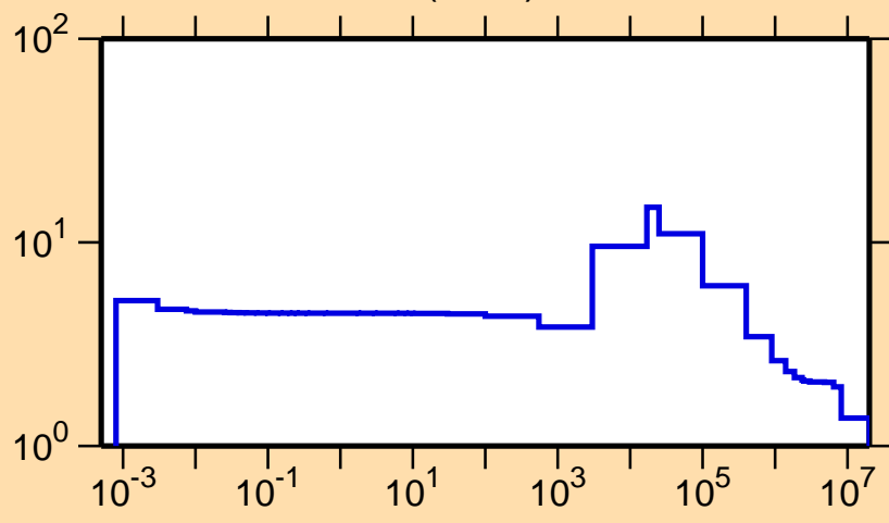
\sigma vs. E for ^{55}\text{Co}(n,\text{el.})
