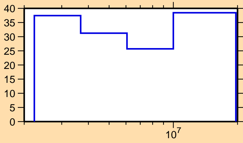
\Delta\sigma/\sigma vs. E for ^{56}\text{Co}(n,ncont.)
