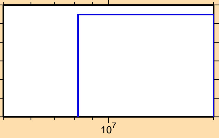
\sigma vs. E for ^{56}\text{Co}(n,2n)
