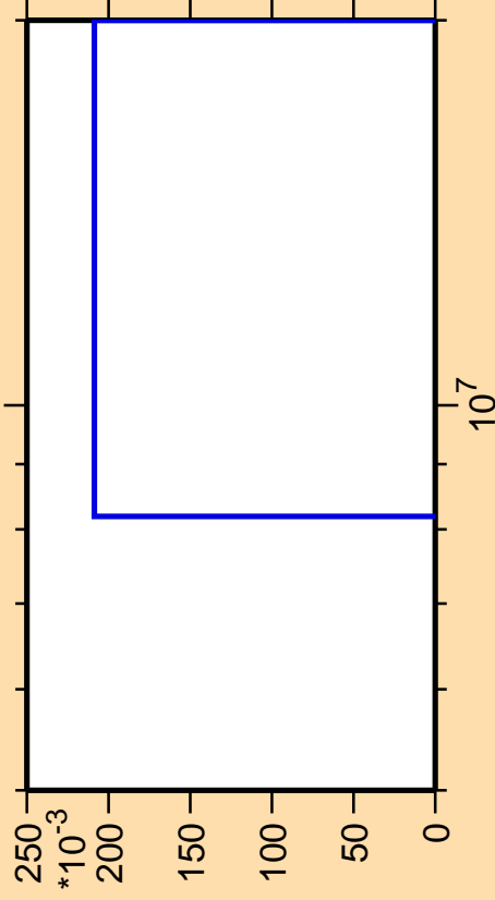
\Delta\sigma/\sigma vs. E for ^{56}\text{Co}(\text{mt } 45)
