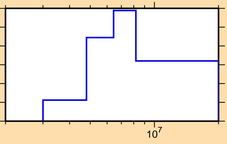
\sigma vs. E for ^{56}\text{Co}(n,n\text{cont.})
