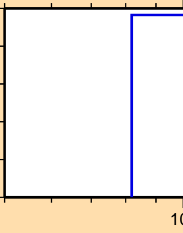
\sigma vs. E for ^{56}\text{Co}(n,\text{nd})
