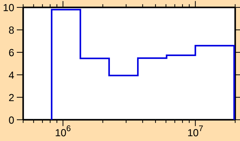
\Delta\sigma/\sigma vs. E for ^{57}\text{Co}(\text{n,nonel.})
