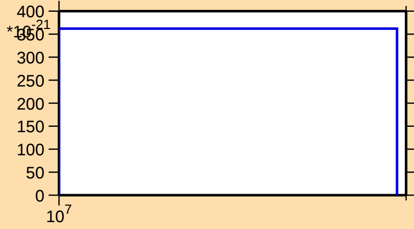
\sigma vs. E for ^{57}\text{Co}(n,2n\alpha)
