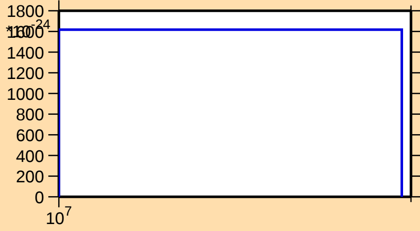
\sigma vs. E for ^{57}\text{Co}(n,\text{pt})
