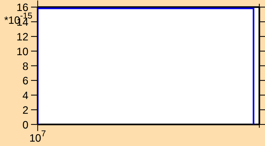
\sigma vs. E for ^{57}\text{Co}(n,\text{nt})
