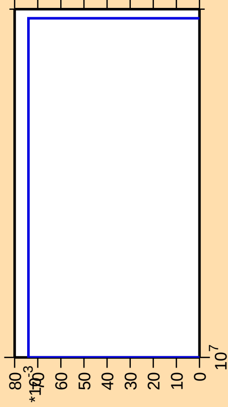
\Delta\sigma/\sigma vs. E for ^{57}\text{Co}(n,\text{nt})
