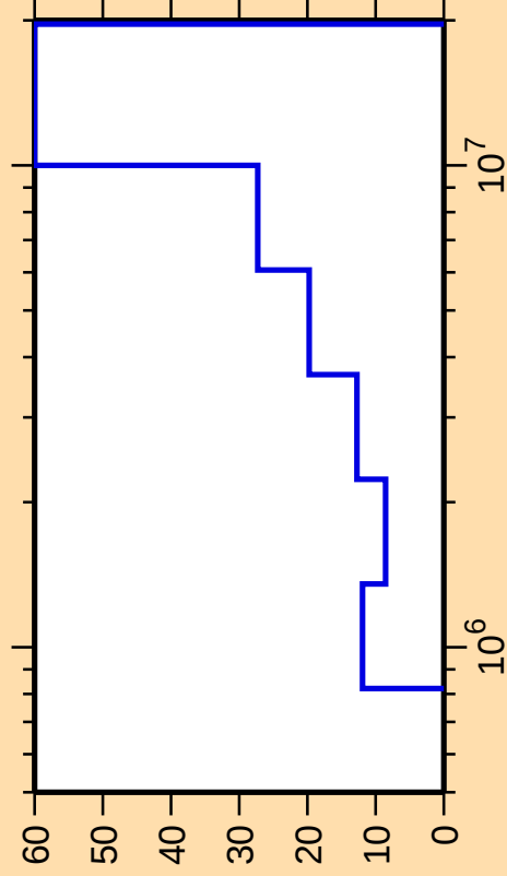
\Delta\sigma/\sigma vs. E for ^{57}\text{Co}(\text{n,inel.})
