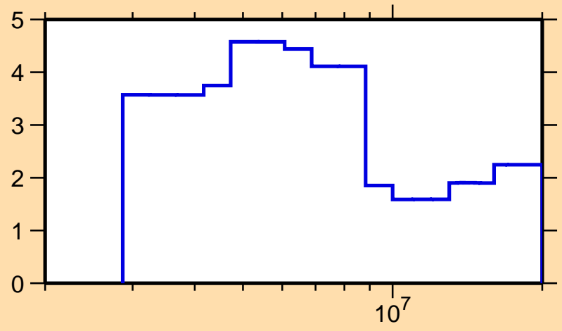
\Delta\sigma/\sigma vs. E for ^{59}\text{Co}(n,n\text{nonel.})
