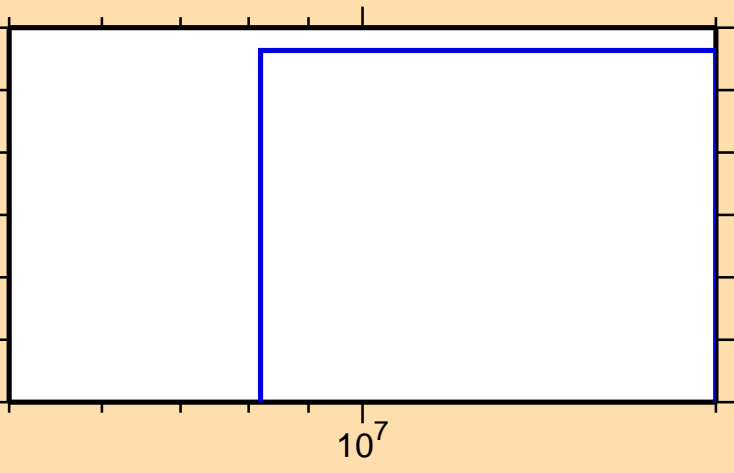
\sigma vs. E for ^{59}\text{Co}(n,\text{He3})
