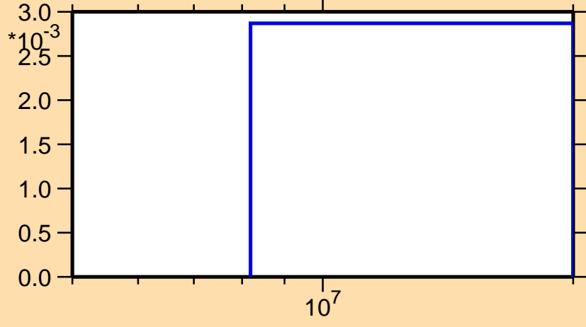
\sigma vs. E for ^{59}\text{Co}(n,n\alpha)
