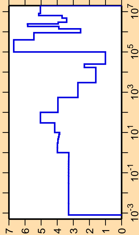
\Delta\sigma/\sigma vs. E for ^{59}\text{Co}(n,\text{el.})
