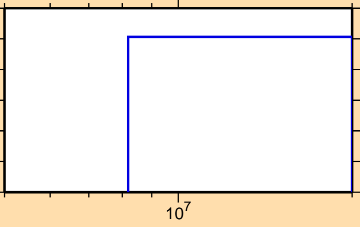
\sigma vs. E for ^{60}\text{Co}(n,p\alpha)
