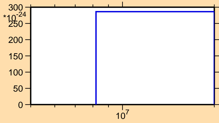
\sigma vs. E for ^{60}\text{Co} (mt 34)
