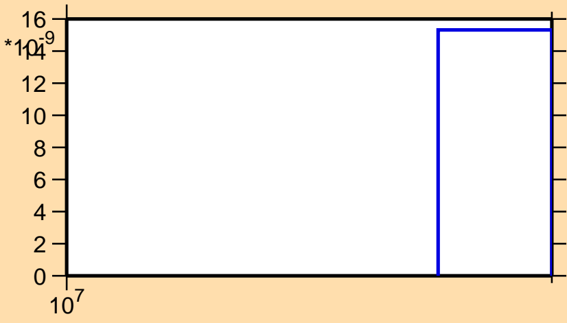
\sigma vs. E for ^{61}\text{Co}(n,2np)
