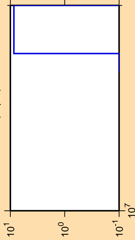
\Delta\sigma/\sigma vs. E for ^{61}\text{Co}(n,p\alpha)
