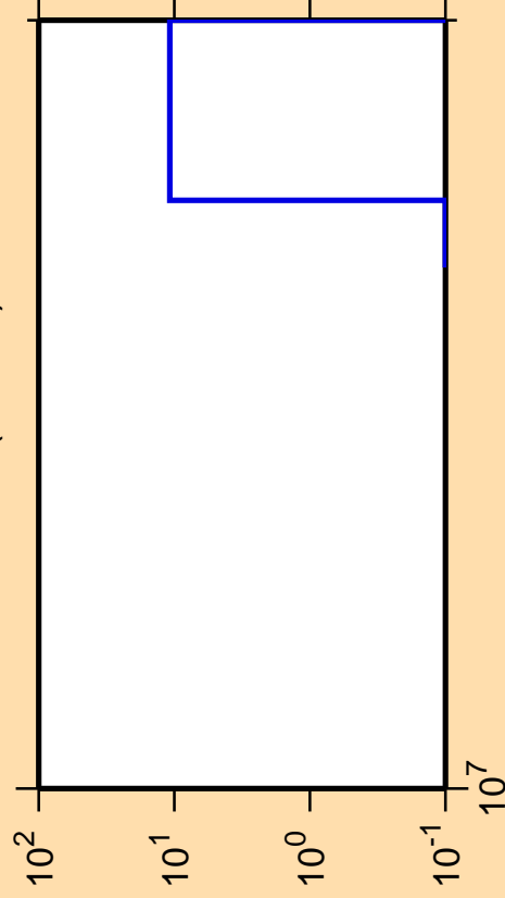
\Delta\sigma/\sigma vs. E for ^{61}\text{Co}(n,\text{He3})
