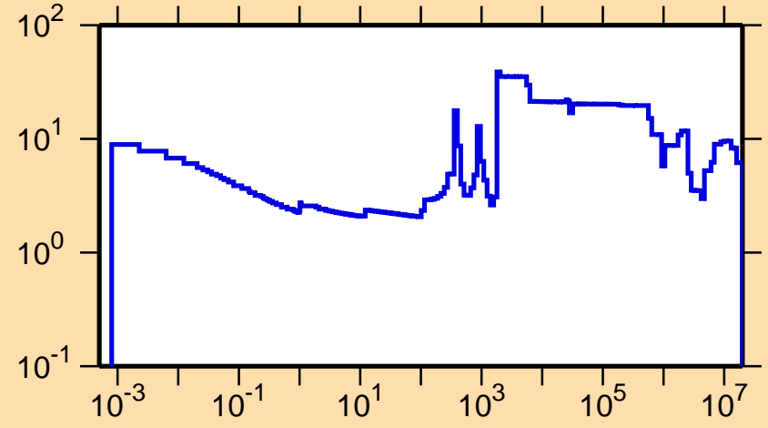
\Delta\sigma/\sigma vs. E for ^{61}\text{Co}(n,\text{tot.})
