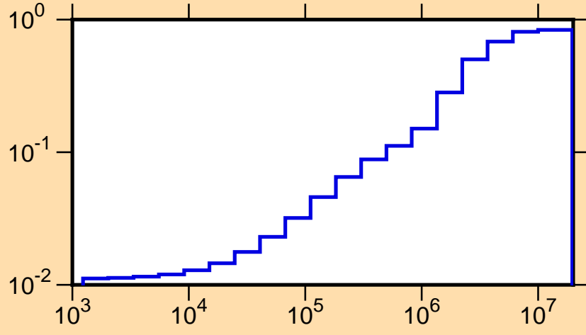
\mu vs. E for ^{61}\text{Co}(\text{mt251})
