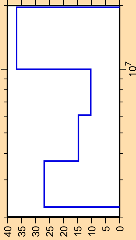
\Delta\sigma/\sigma vs. E for ^{61}\text{Co}(n,n\text{cont.})
