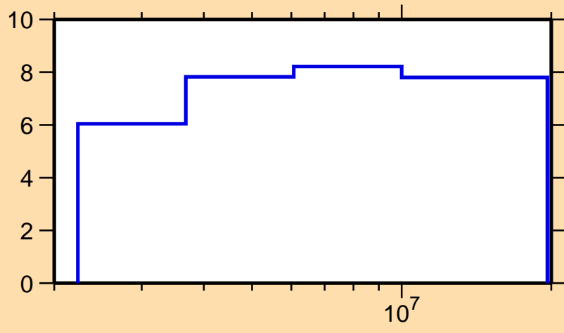
\Delta\sigma/\sigma vs. E for ^{61}\text{Co}(n,n\text{nonel.})
