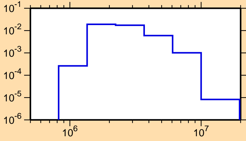
\sigma vs. E for ^{61}\text{Co}(n,n_3)
