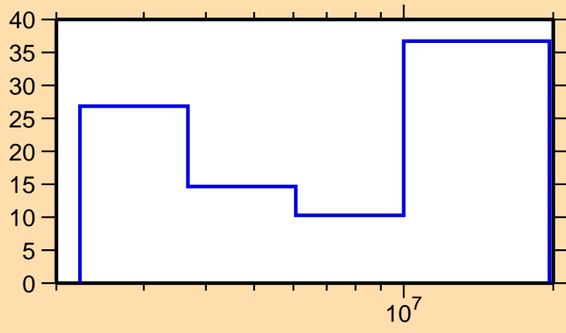
\Delta\sigma/\sigma vs. E for ^{61}\text{Co}(n,n\text{cont.})
