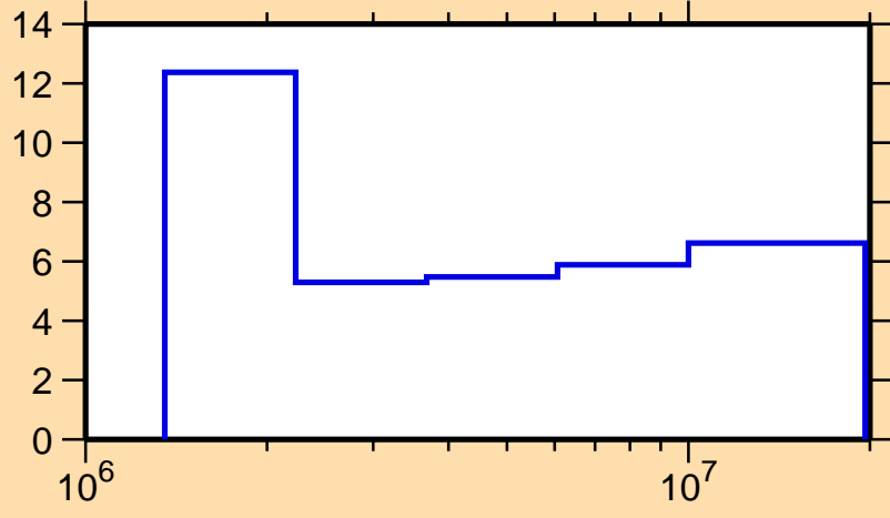
\Delta\sigma/\sigma vs. E for ^{62}\text{Co}(n,n\text{nonel.})
