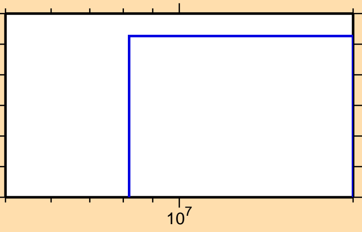
\sigma vs. E for ^{62}\text{Co}(n,2np)
