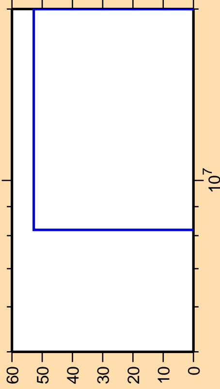
\Delta\sigma/\sigma vs. E for ^{62}\text{Co}(n,n\alpha)
