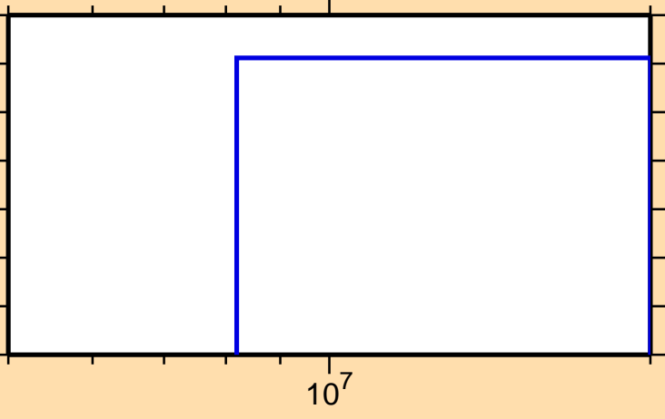
\sigma vs. E for ^{62}\text{Co}(n,np)
