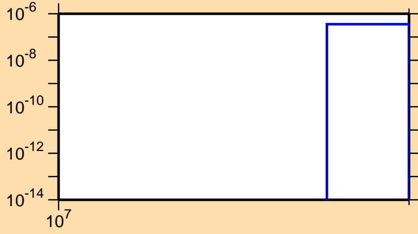
\sigma vs. E for ^{63}\text{Co}(n,\text{nd})
