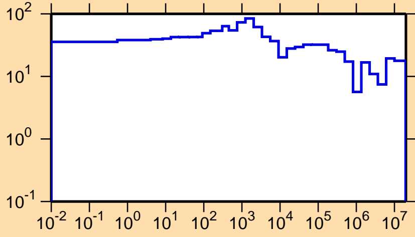
\Delta\sigma/\sigma vs. E for ^{63}\text{Co}(n,\text{el.})
