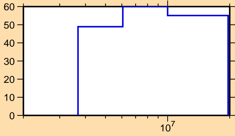
\Delta\sigma/\sigma vs. E for ^{63}\text{Co}(n,n_1)
