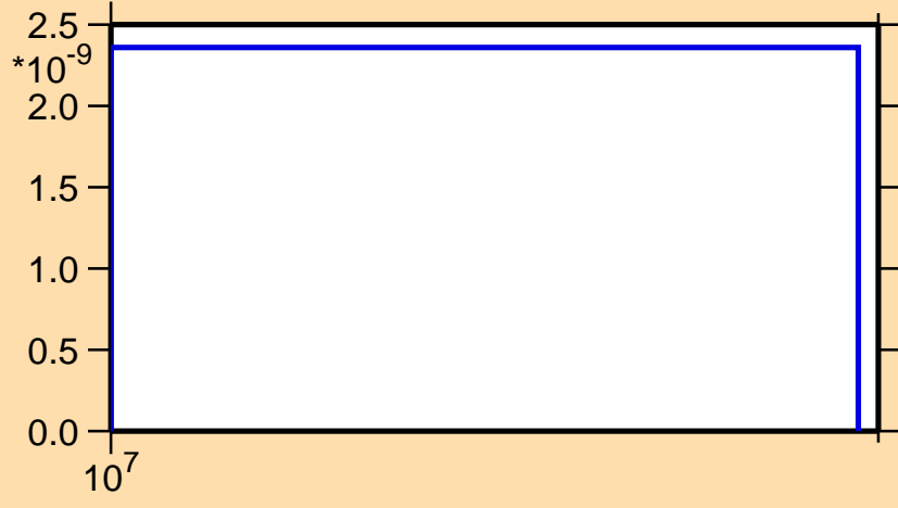
\sigma vs. E for ^{63}\text{Co}(n,\text{nd})
