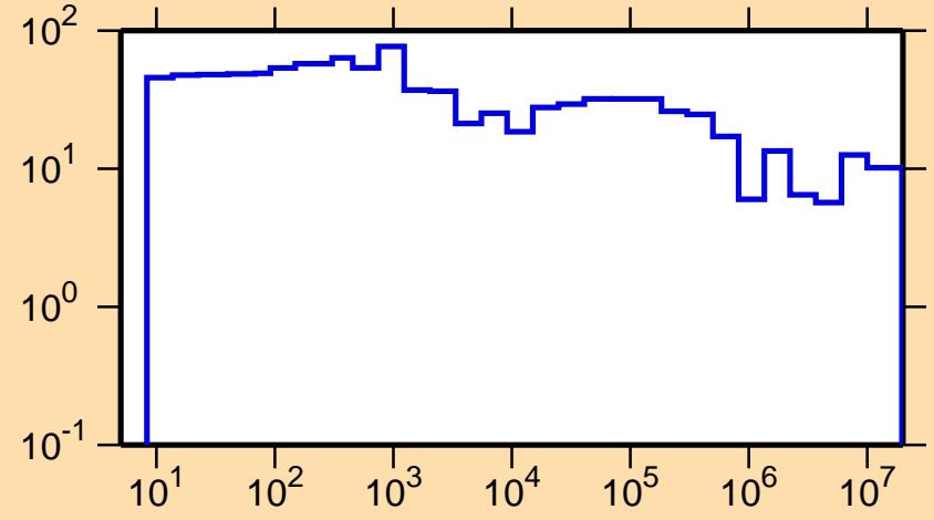
\Delta\sigma/\sigma vs. E for ^{63}\text{Co}(n,\text{tot.})
