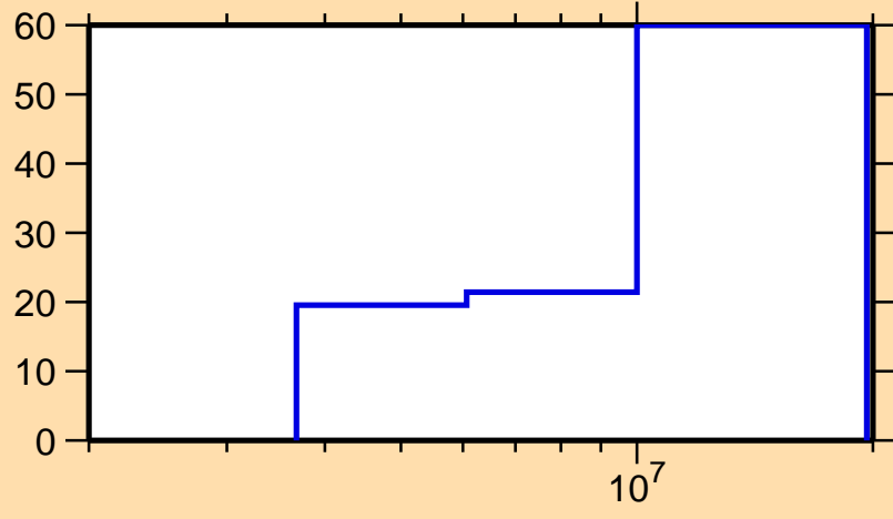
\Delta\sigma/\sigma vs. E for ^{63}\text{Co}(n,\gamma)
