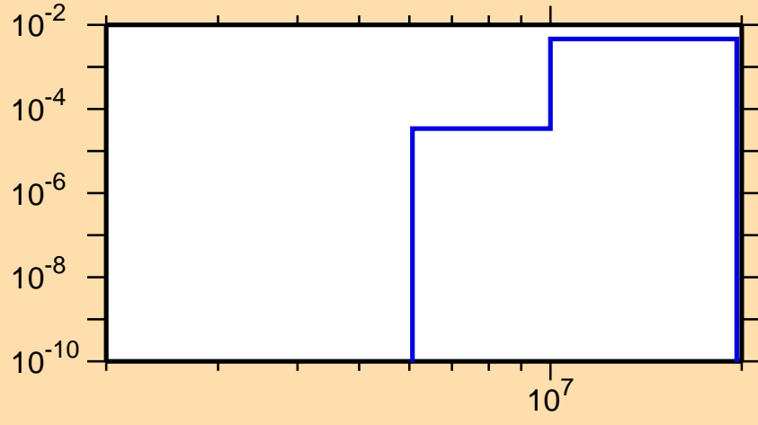
\sigma vs. E for ^{63}\text{Co}(n,p)
