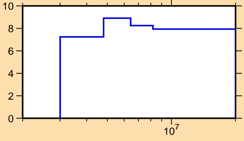
\Delta\sigma/\sigma vs. E for ^{63}\text{Co}(n,n\text{nonel.})
