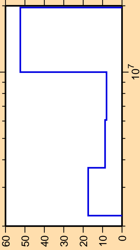
\Delta\sigma/\sigma vs. E for ^{65}\text{Co}(n,n_{\text{cont}})
