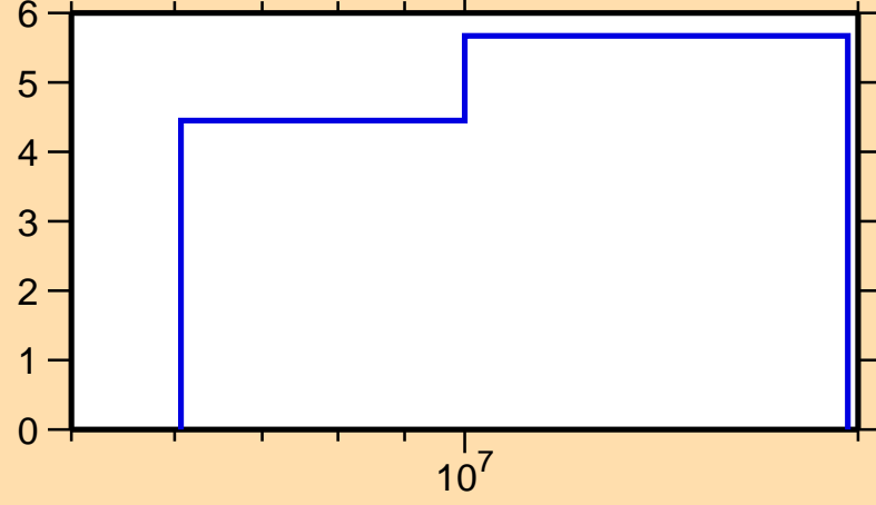
\Delta\sigma/\sigma vs. E for ^{65}\text{Co}(n,\text{el.})
