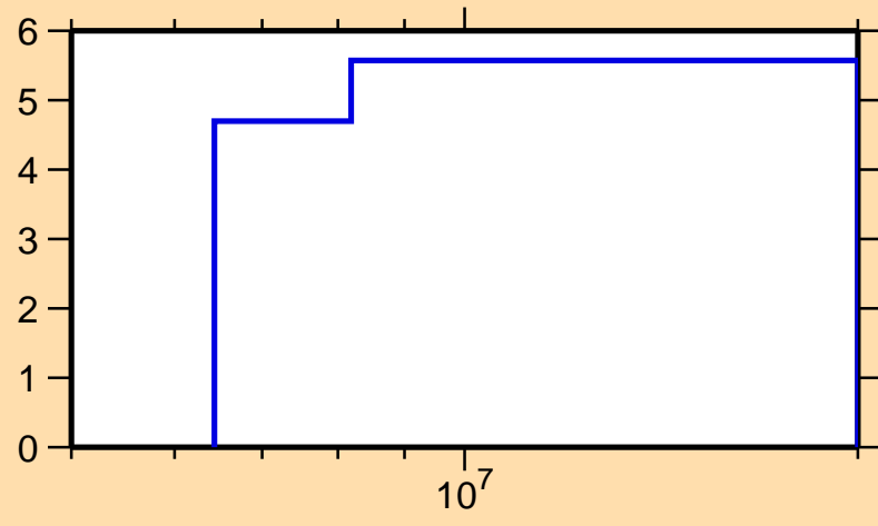
\Delta\sigma/\sigma vs. E for ^{65}\text{Co}(n,el.)
