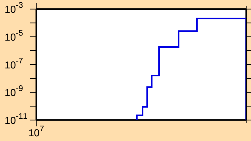
\sigma vs. E for ^{68}\text{Co}(n,np)
