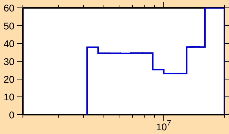
\Delta\sigma/\sigma vs. E for ^{68}\text{Co}(n,2n)
