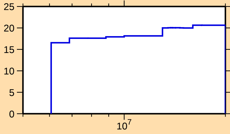
\Delta\sigma/\sigma vs. E for ^{68}\text{Co}(n,\text{nonel.})
