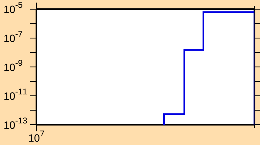
\sigma vs. E for ^{68}\text{Co}(n,\text{nd})
