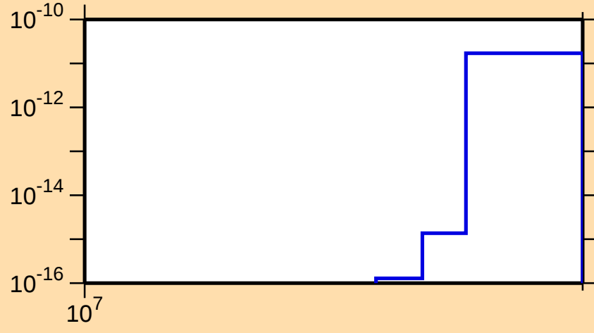
\sigma vs. E for ^{68}\text{Co}(n,2n\alpha)
