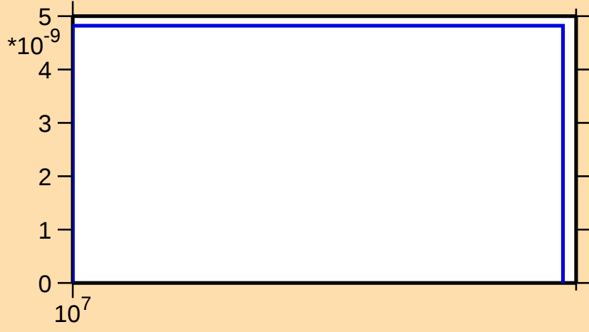
\sigma vs. E for ^{68}\text{Co}(n,\text{nt})
