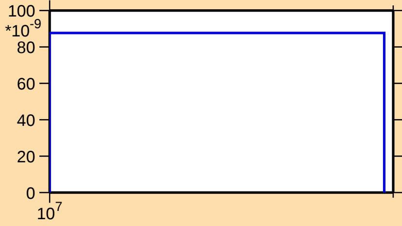
\sigma vs. E for ^{68}\text{Co}(n,n\alpha)
