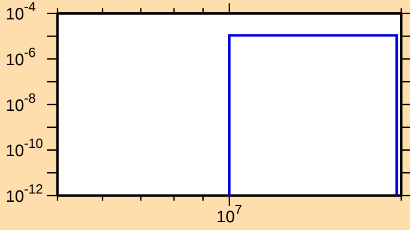
\sigma vs. E for ^{68}\text{Co}(n,t)
