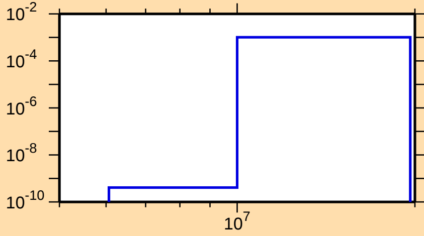
\sigma vs. E for ^{68}\text{Co}(n,p)
