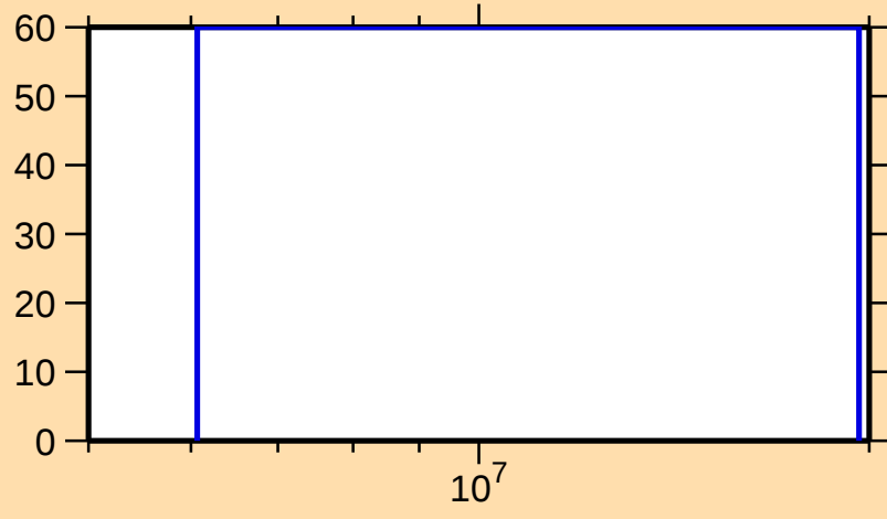
\Delta\sigma/\sigma vs. E for ^{68}\text{Co}(n,n\text{cont.})
