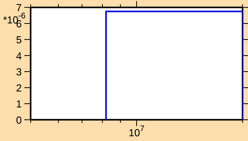
\sigma vs. E for ^{68}\text{Co}(n,d)
