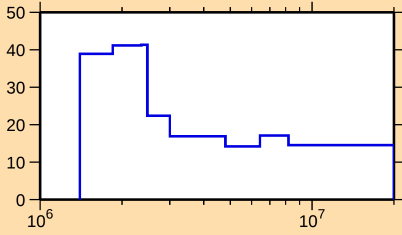
\Delta\sigma/\sigma vs. E for ^{68}\text{Co}(n,\text{el.})
