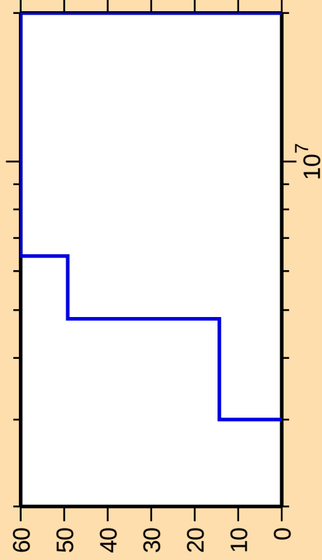
\Delta\sigma/\sigma vs. E for ^{68}\text{Co}(n,n_{\text{cont}}) .
