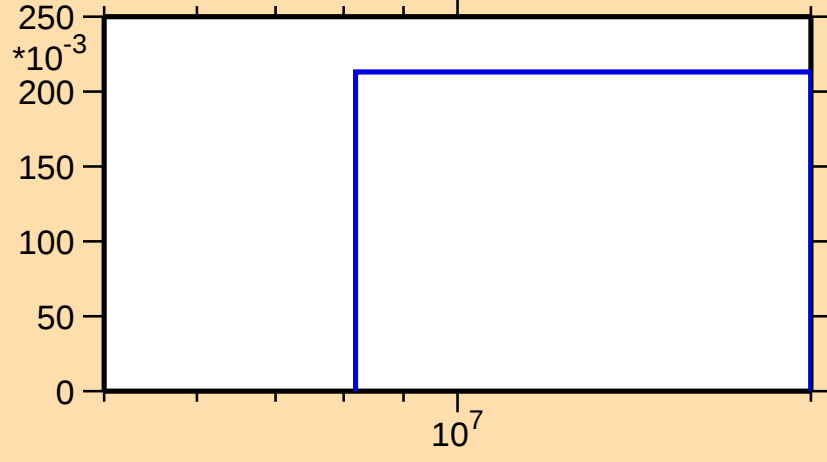
\sigma vs. E for ^{68}\text{Co}(n,3n)
