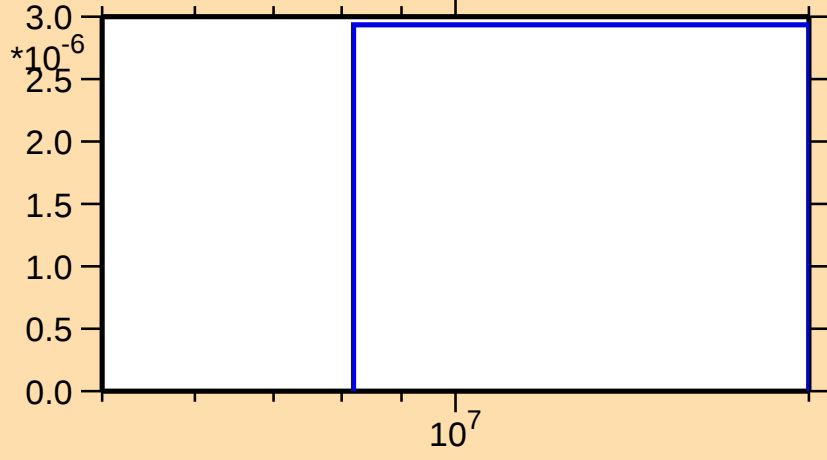
\sigma vs. E for ^{68}\text{Co}(n,np)
