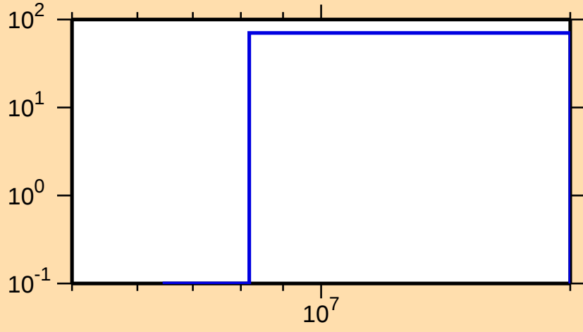
\Delta\sigma/\sigma vs. E for ^{68}\text{Co}(n,p)
