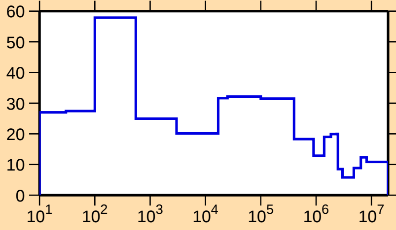
\Delta\sigma/\sigma vs. E for ^{68}\text{Co}(n,\text{tot.})
