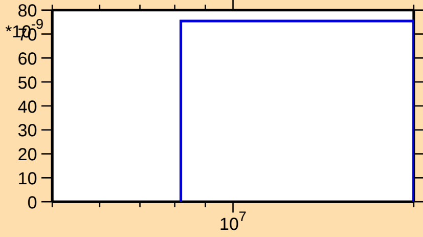
\sigma vs. E for ^{68}\text{Co}(n,n\alpha)
