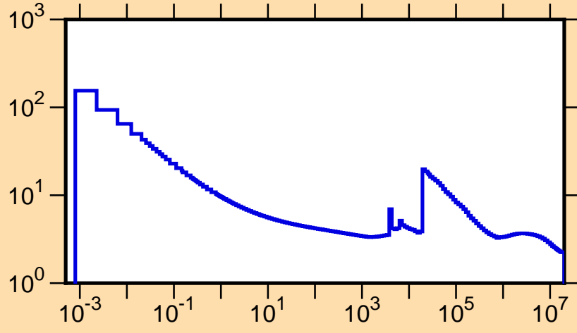
\sigma vs. E for ^{48}\text{Cr}(n,\text{tot.})
