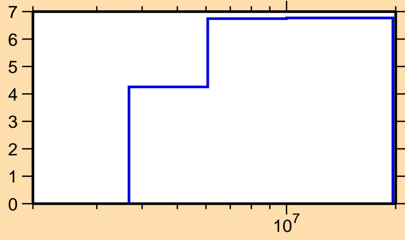
\Delta\sigma/\sigma vs. E for ^{48}\text{Cr}(n,tot.)
