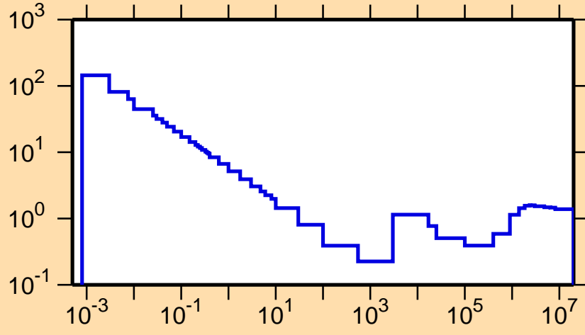
\sigma vs. E for ^{48}\text{Cr}(n,\text{nonel.})
