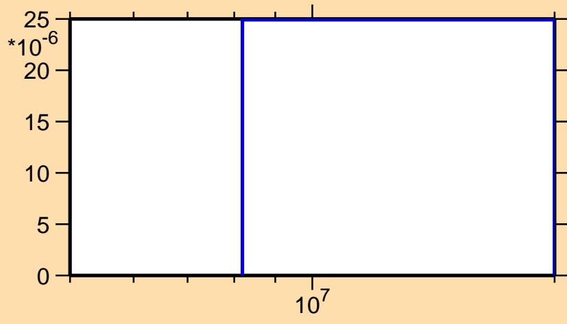
\sigma vs. E for ^{48}\text{Cr}(n,\text{pd})
