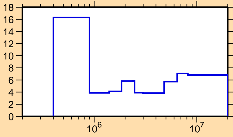
\Delta\sigma/\sigma vs. E for ^{48}\text{Cr}(n,\text{tot.})
