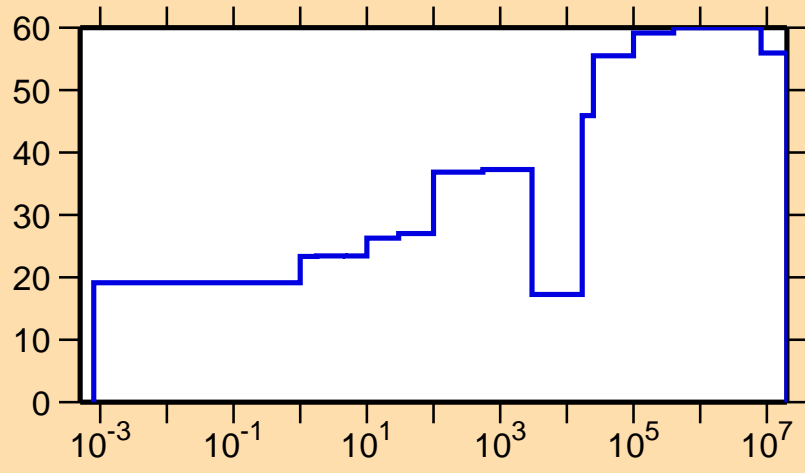
\Delta\sigma/\sigma vs. E for ^{48}\text{Cr}(n,\gamma)
