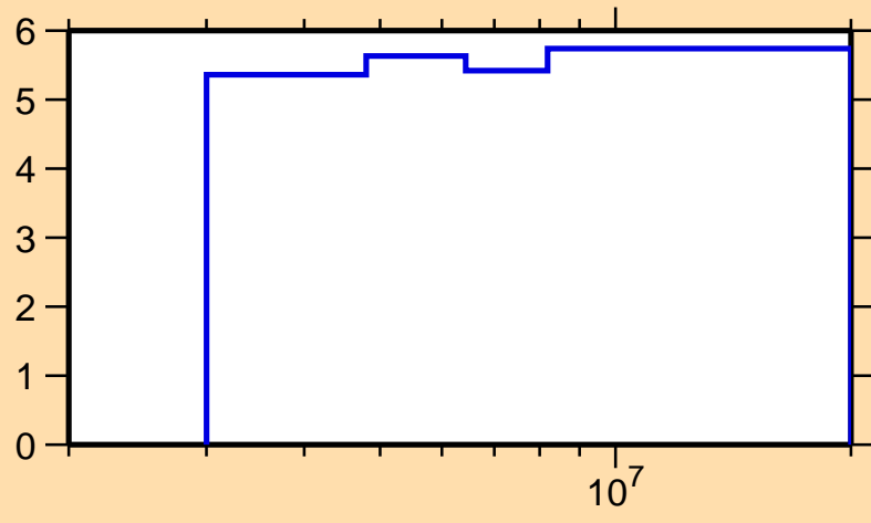
\Delta\sigma/\sigma vs. E for ^{48}\text{Cr}(n,\text{nonel.})
