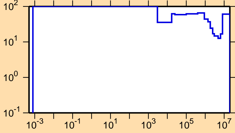
\Delta\sigma/\sigma vs. E for ^{48}\text{Cr}(n,p)
