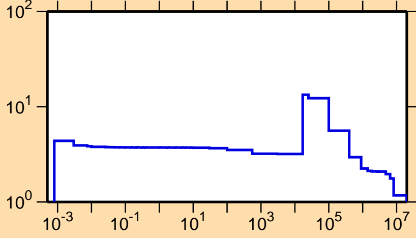
\sigma vs. E for ^{48}\text{Cr}(n,\text{el.})
