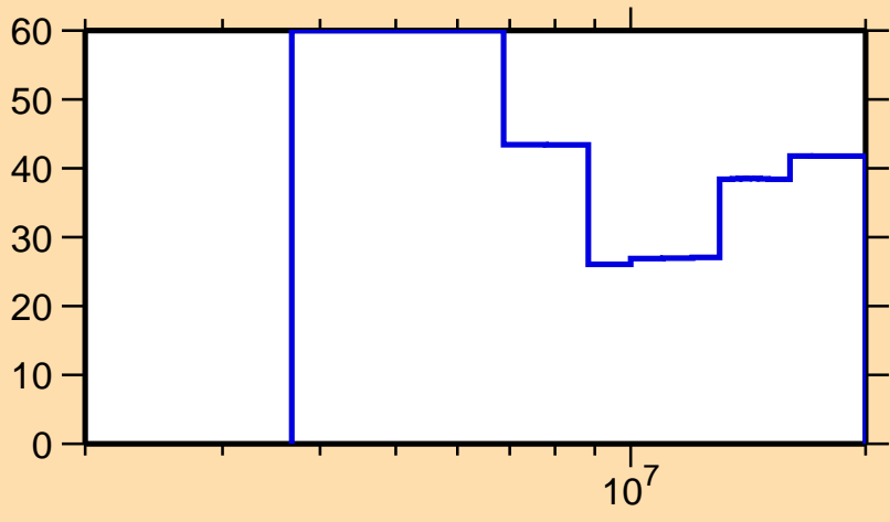
\Delta\sigma/\sigma vs. E for ^{49}\text{Cr}(n,n\text{cont.})
