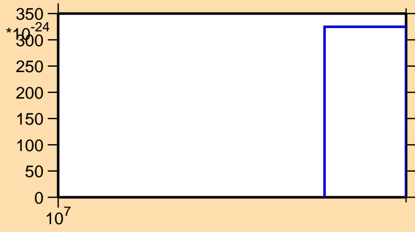
\sigma vs. E for ^{49}\text{Cr}(n,2n\alpha)
