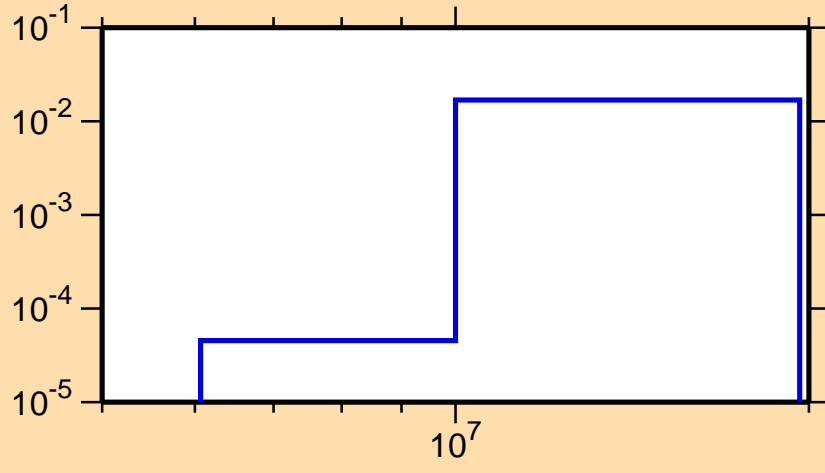
\sigma vs. E for ^{49}\text{Cr}(n,d)
