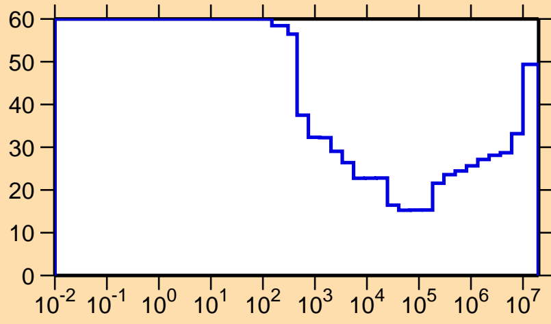
\Delta\sigma/\sigma vs. E for ^{49}\text{Cr}(n,p)
