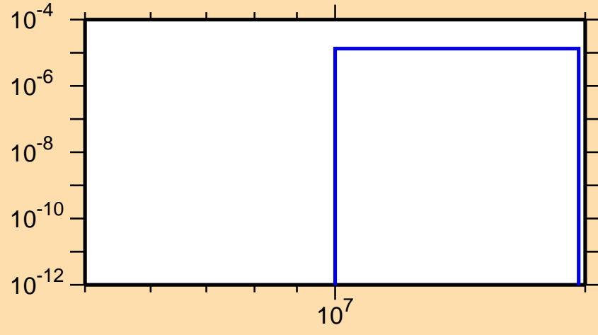
\sigma vs. E for ^{49}\text{Cr}(n,\text{He}3)
