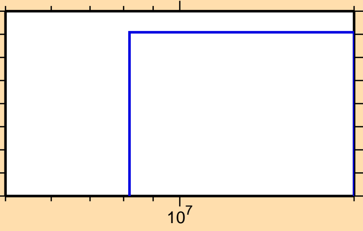
\sigma vs. E for ^{50}\text{Cr}(n,\text{He}3)
