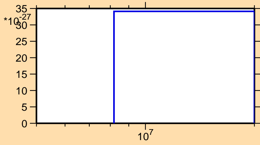
\sigma vs. E for ^{50}\text{Cr}(n,\text{pt})
