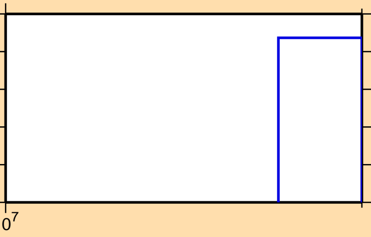
\sigma vs. E for ^{51}\text{Cr}(n,2n\alpha)
