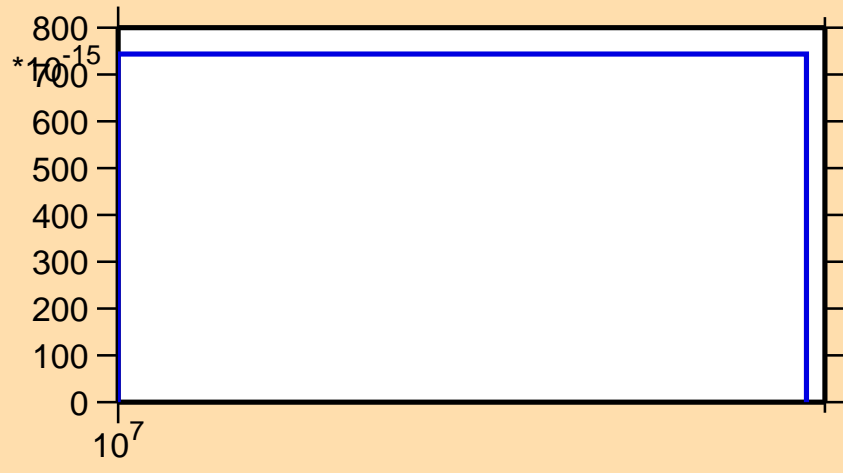
\sigma vs. E for ^{51}\text{Cr}(n,2np)
