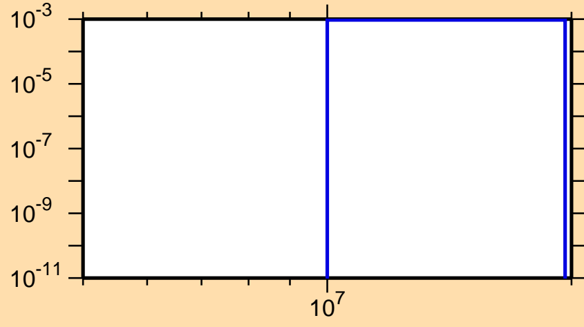
\sigma vs. E for ^{51}\text{Cr}(n,\alpha)
